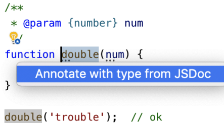
Figure 10-5. Quick fix to copy JSDoc annotations to TypeScript type annotations.
