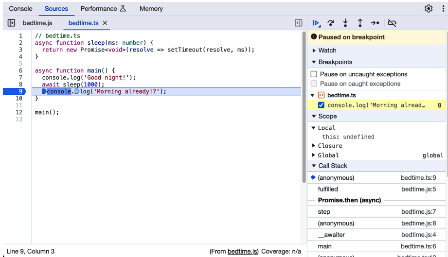
Figure 9-7. Debugging the original TypeScript source for a Node.js program.
