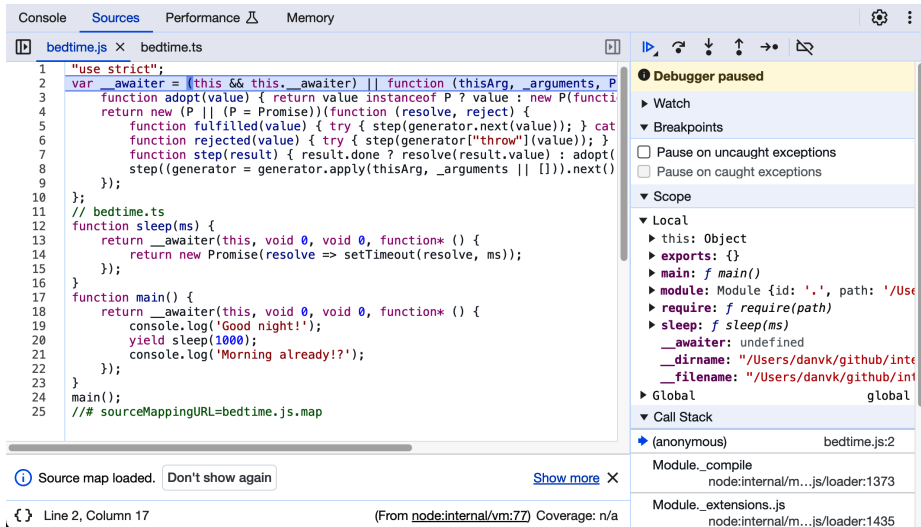
Figure 9-6. Generated JavaScript for a Node.js program in Google Chrome Devtools. Note the source map reference at the bottom.
