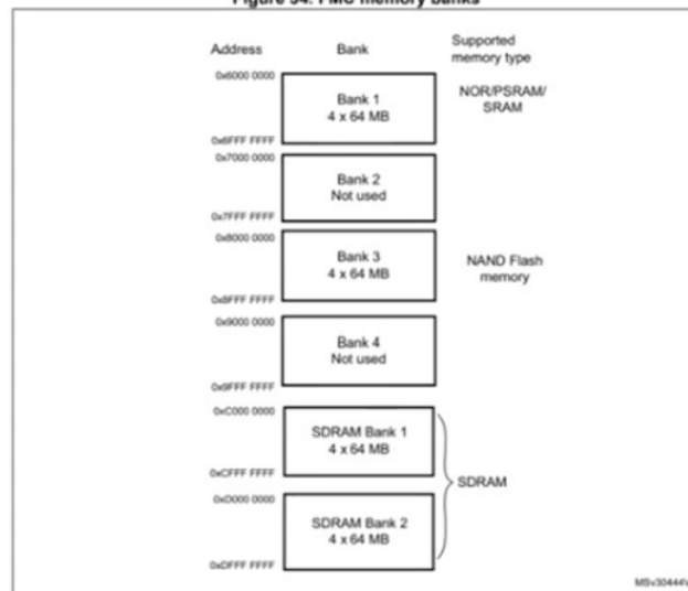
Figure 34. FMC memory banks
