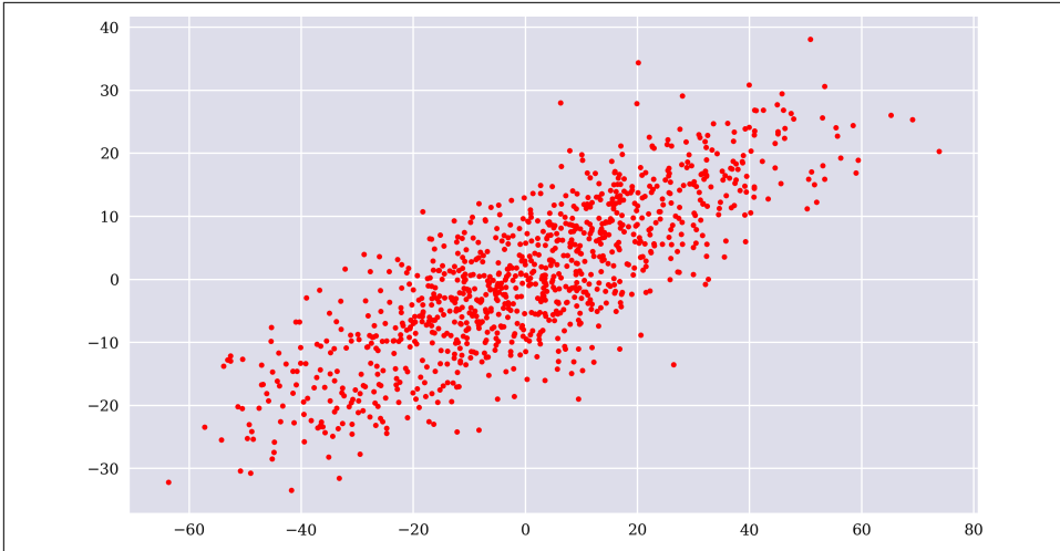
Figure 2-4. The random portfolios spanning a two-dimensional area (around the origin)
