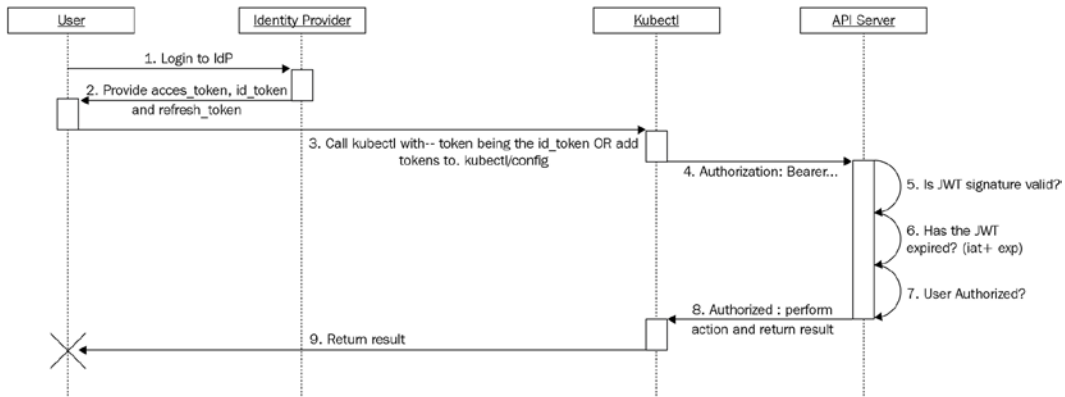
Figure 7.1 – Kubernetes/kubectl OpenID Connect sequence diagram
