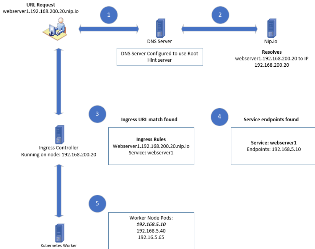
Figure 6.5 – Ingress traffic flow
