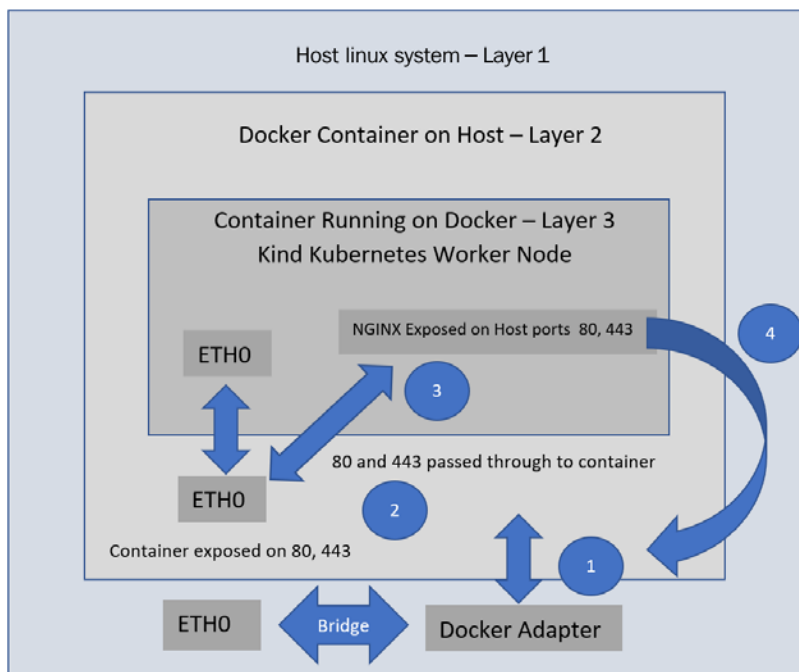
Figure 4.5 – Host communicates with KinD via an Ingress controller
