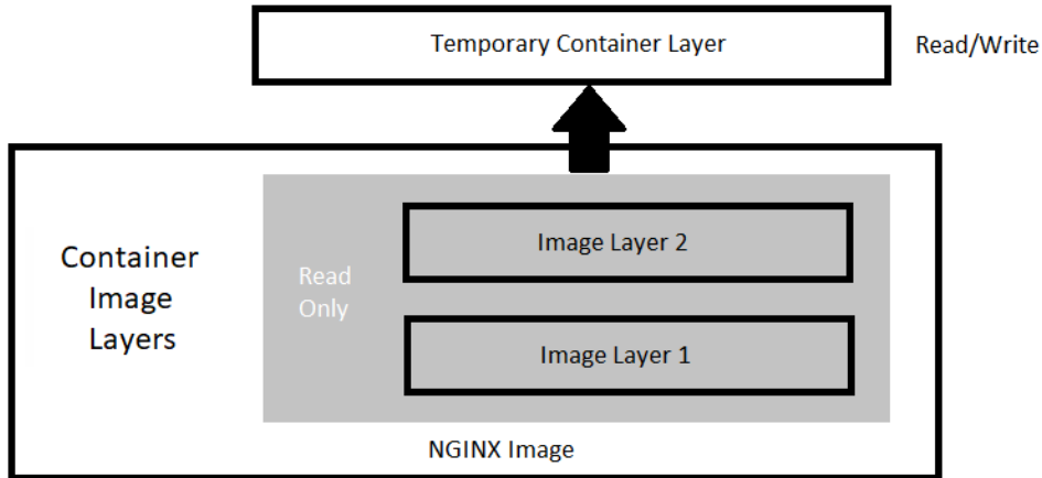
Figure 1.1 – Docker image layers
