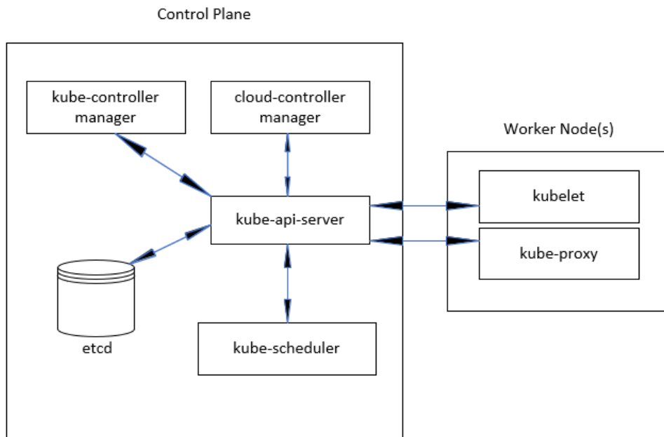
Figure 5.1 – Kubernetes cluster components
