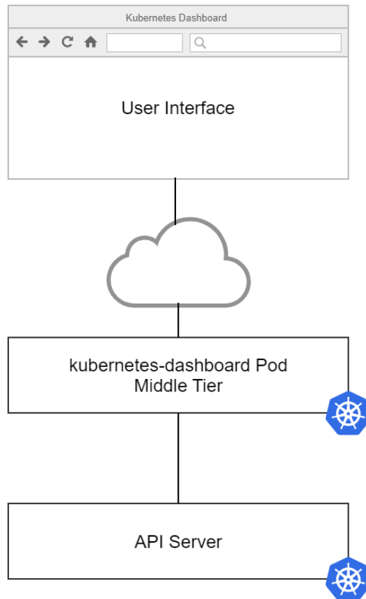
Figure 9.1 – Kubernetes Dashboard architecture
