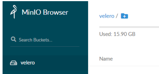
Figure 13.4 – MinIO Browser
