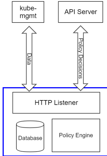
Figure 11.2 – OPA in Kubernetes
