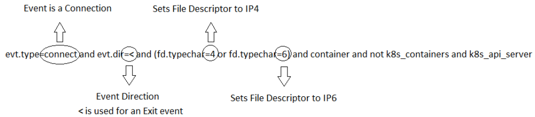
Figure 12.3 – Values in conditions
