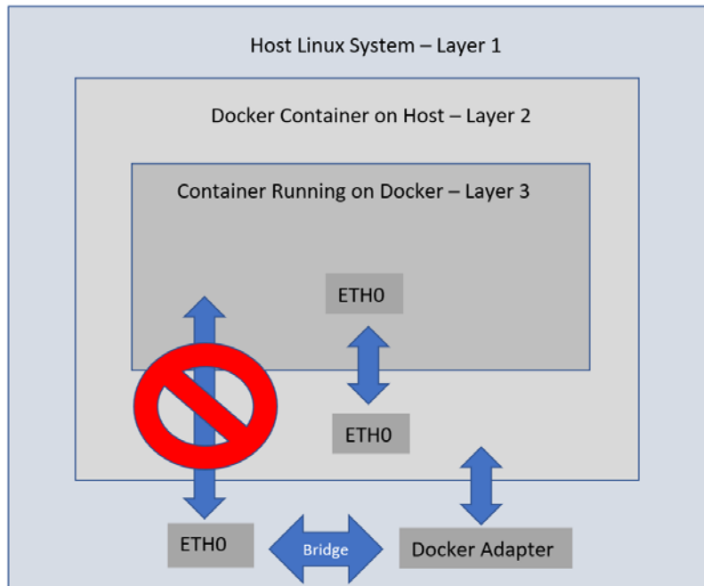
Figure 4.4 – Host cannot communicate with KinD directly
