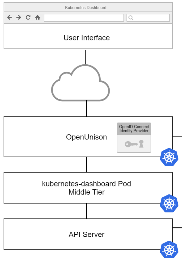
Figure 9.8 – OpenUnison integration with the dashboard
