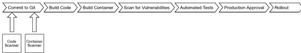
Figure 14.3 – Pipeline with scanners integrated
