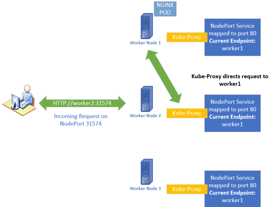
Figure 6.2 – NodePort traffic flow overview
