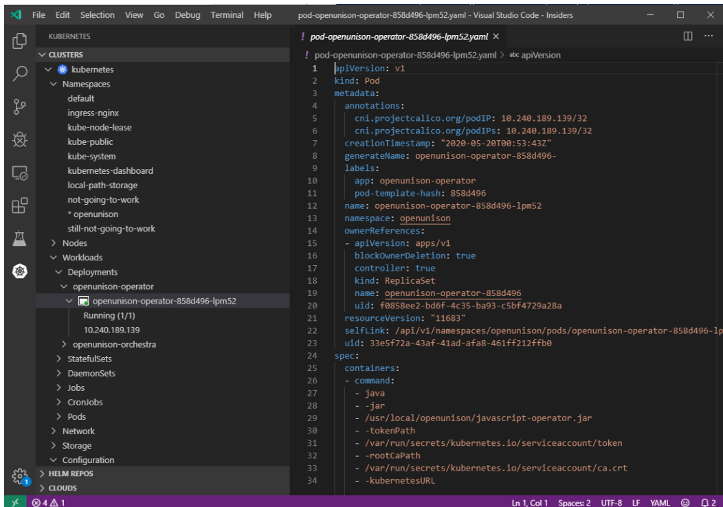
Figure 9.7 – Visual Studio Code with the Kubernetes plugin
