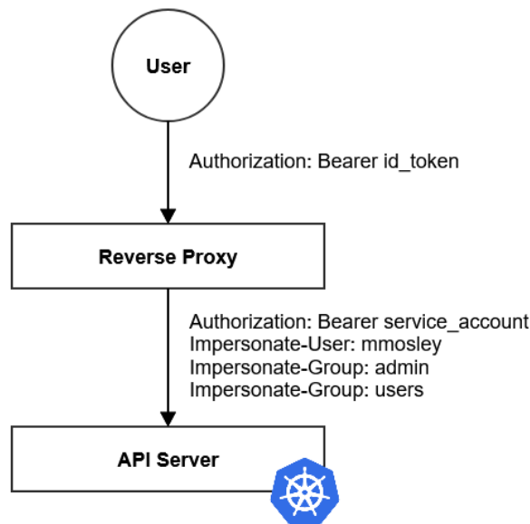
Figure 7.11 – Diagram of how a user interacts with the API server when using Impersonation
