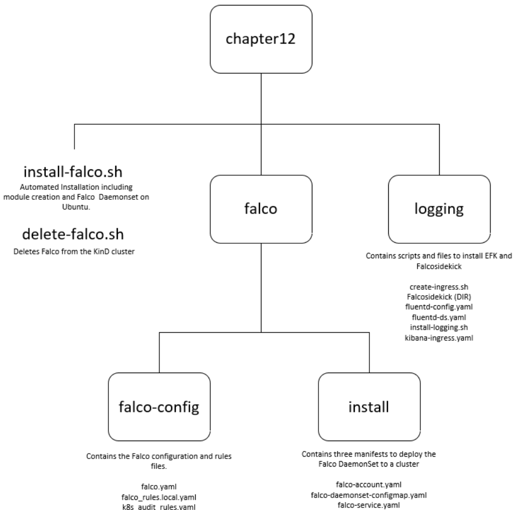
Figure 12.5 – Diagram of the chapter12 directory in the book's GitHub repository
