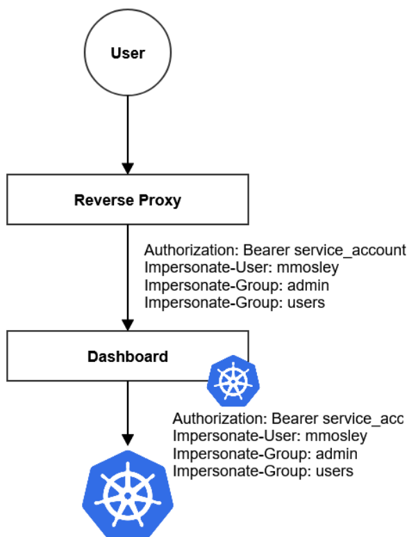
Figure 7.12 – Kubernetes Dashboard with Impersonation
