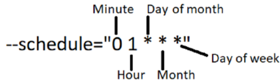
Figure 13.7 – Cron scheduling expression
