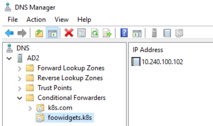
Figure 6.18 – Windows conditional forwarder setup
