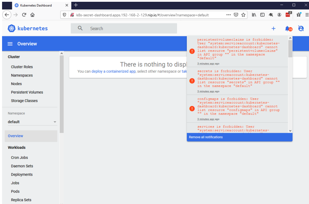
Figure 9.4 – Kubernetes Dashboard with the default service account
