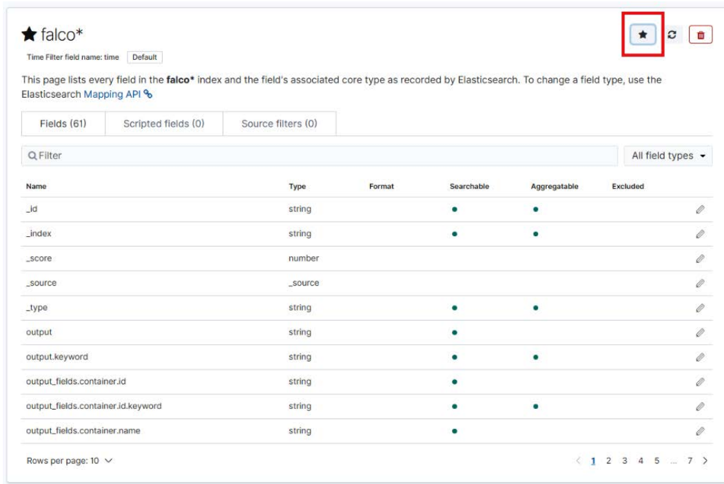
Figure 12.15 – Setting a default index
