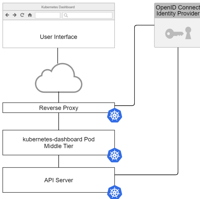
Figure 9.6 – Kubernetes Dashboard with a reverse proxy
