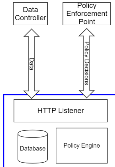
Figure 11.1 – OPA architecture
