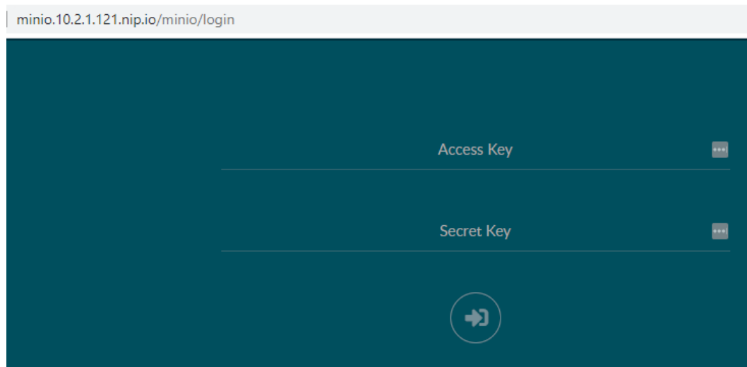
Figure 13.3 – MinIO dashboard
