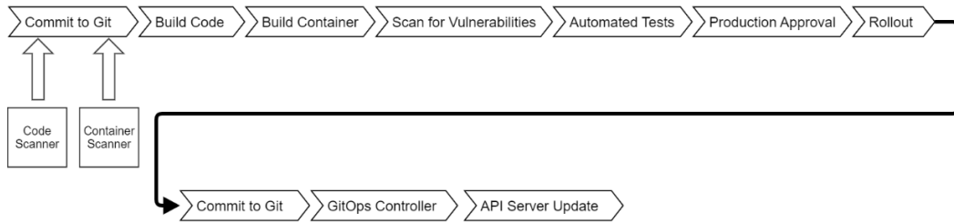
Figure 14.4 – GitOps pipeline
