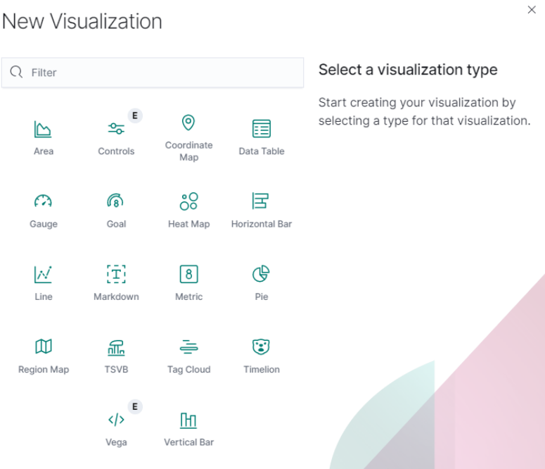
Figure 12.18 – Falco visualizations
