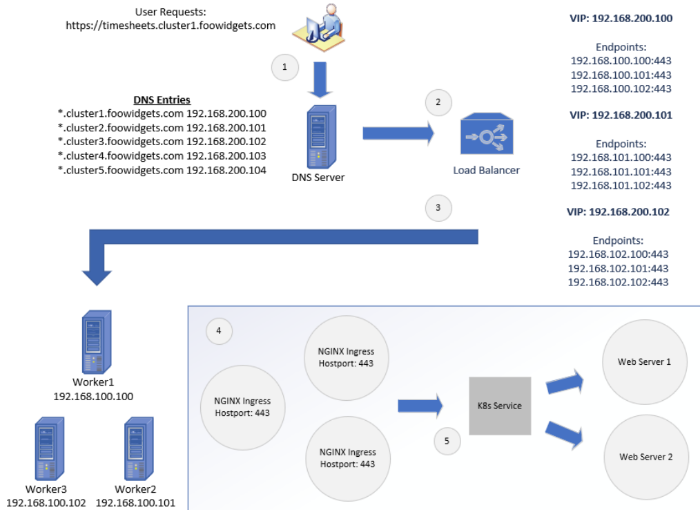
Figure 6.3 – Multiple-name Ingress traffic flow
