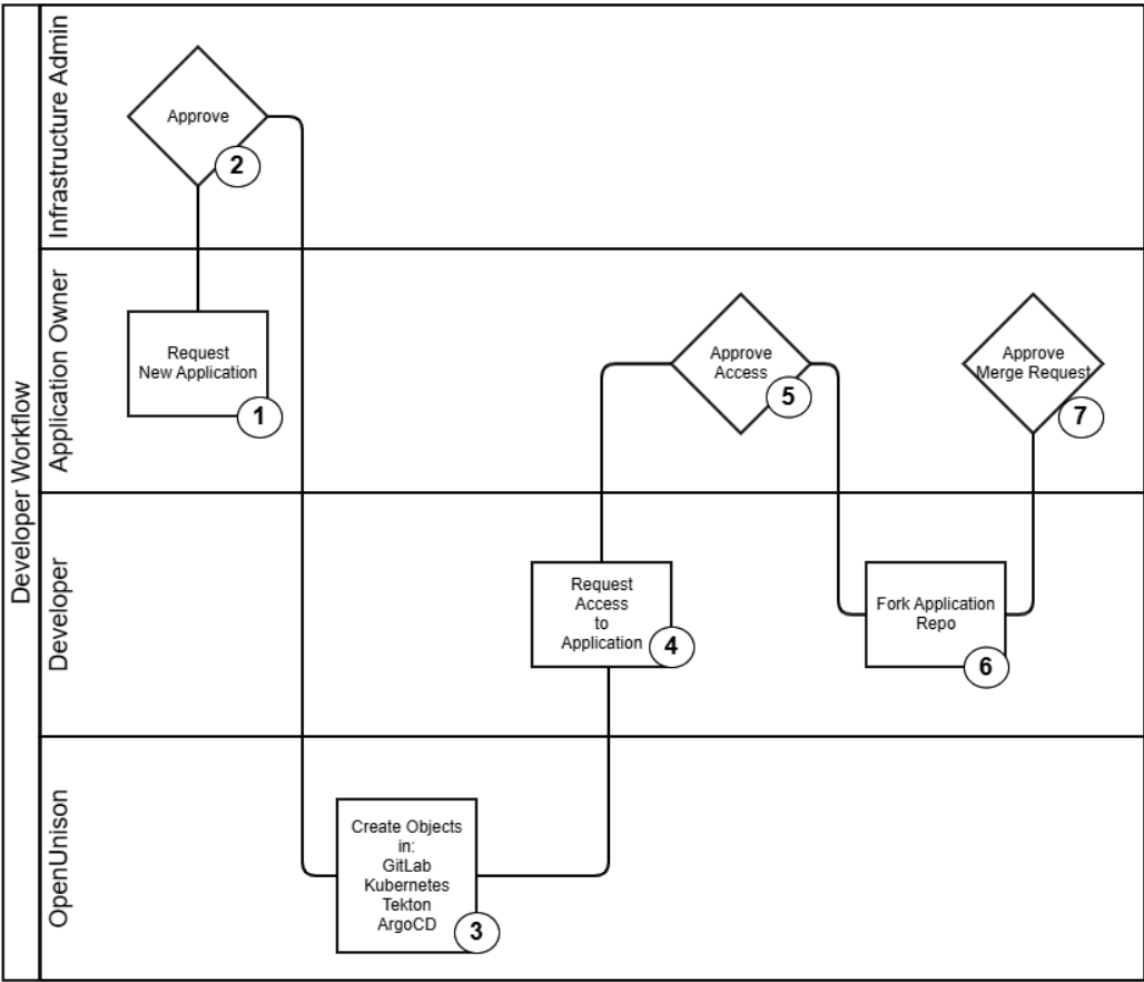
Figure 14.6 – Platform developer workflow
