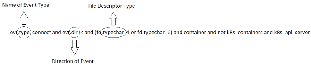
Figure 12.2 – Class Field Value
