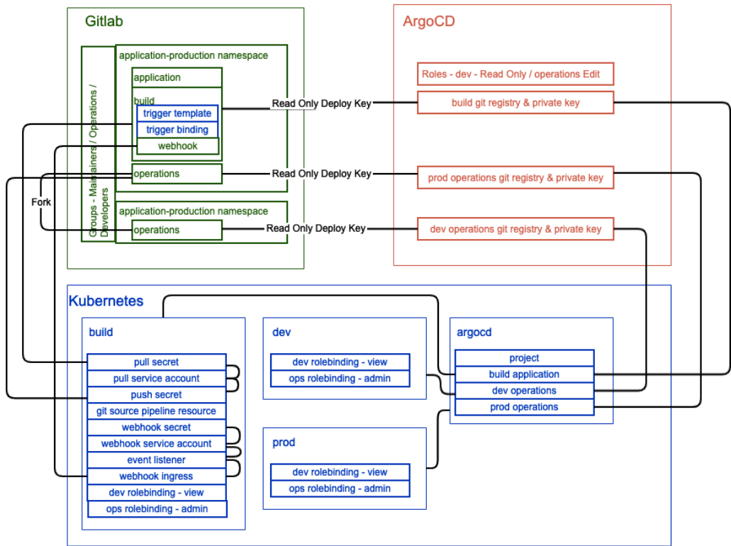
Figure 14.7 – Application onboarding object map
