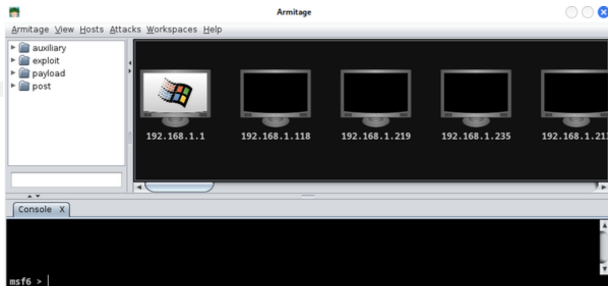
Figure 5-1. Main Armitage window
