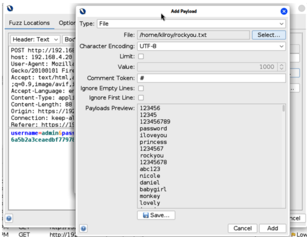
Figure 9-5. ZAP fuzzing attack
