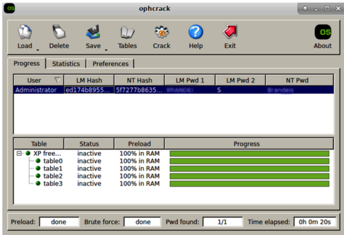
Figure 9-2. Cracked passwords from ophcrack
