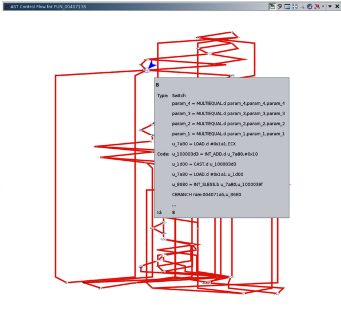
Figure 11-11. Control flow graph in Ghidra
