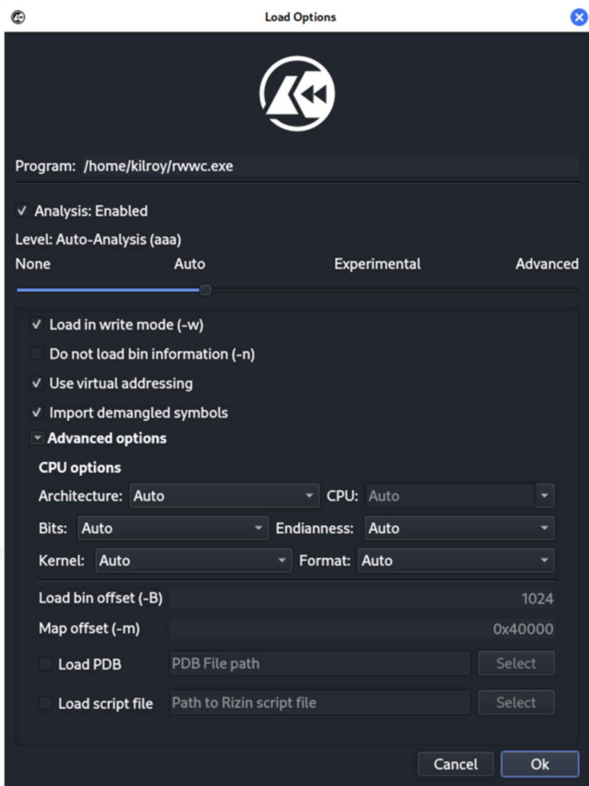
Figure 11-5. Open dialog in Cutter
