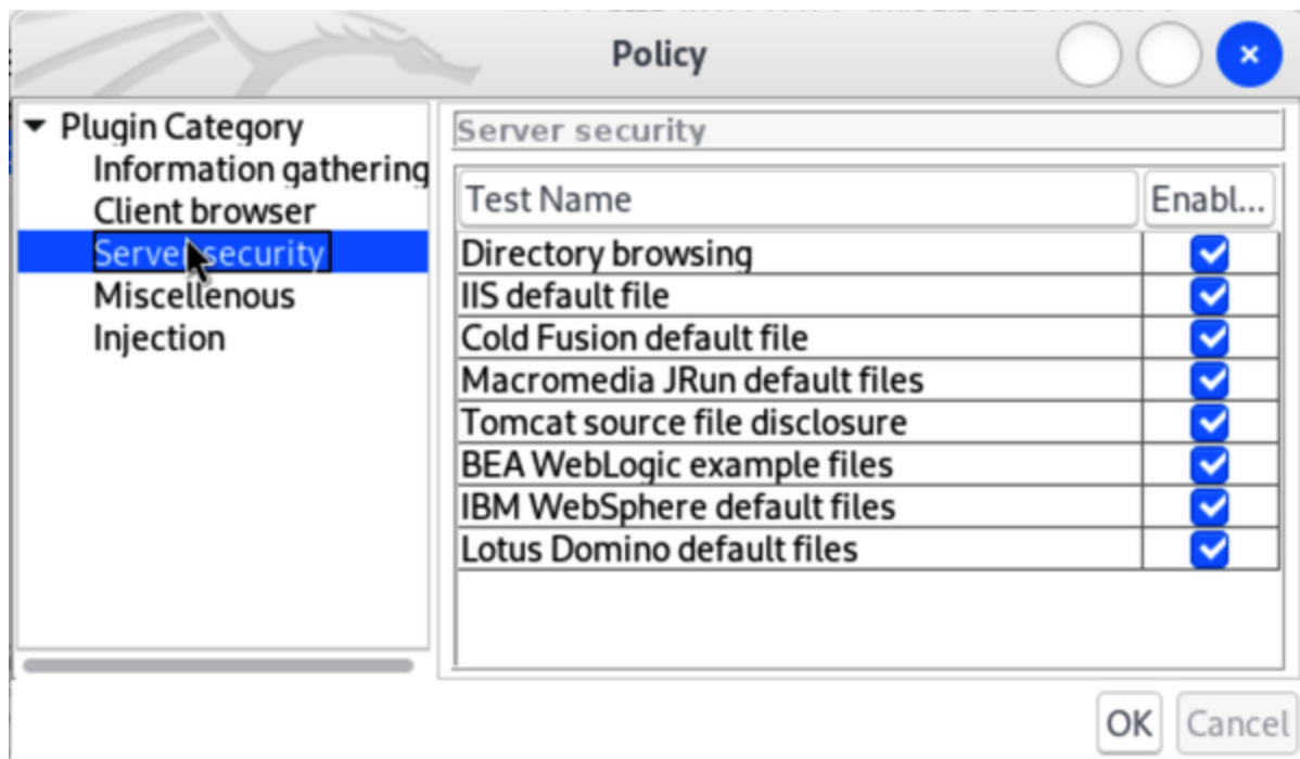
Figure 8-12. Paros policy configuration
