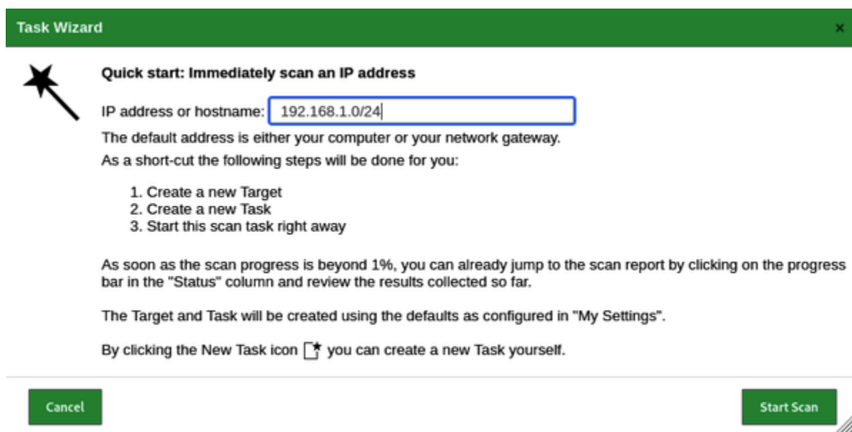
Figure 4-8. Task Wizard
