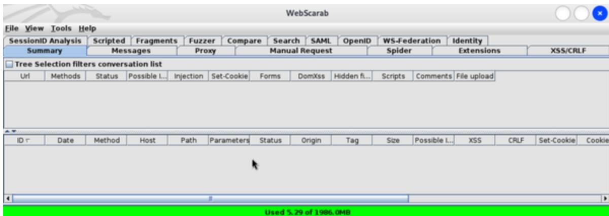
Figure 8-11. WebScarab
