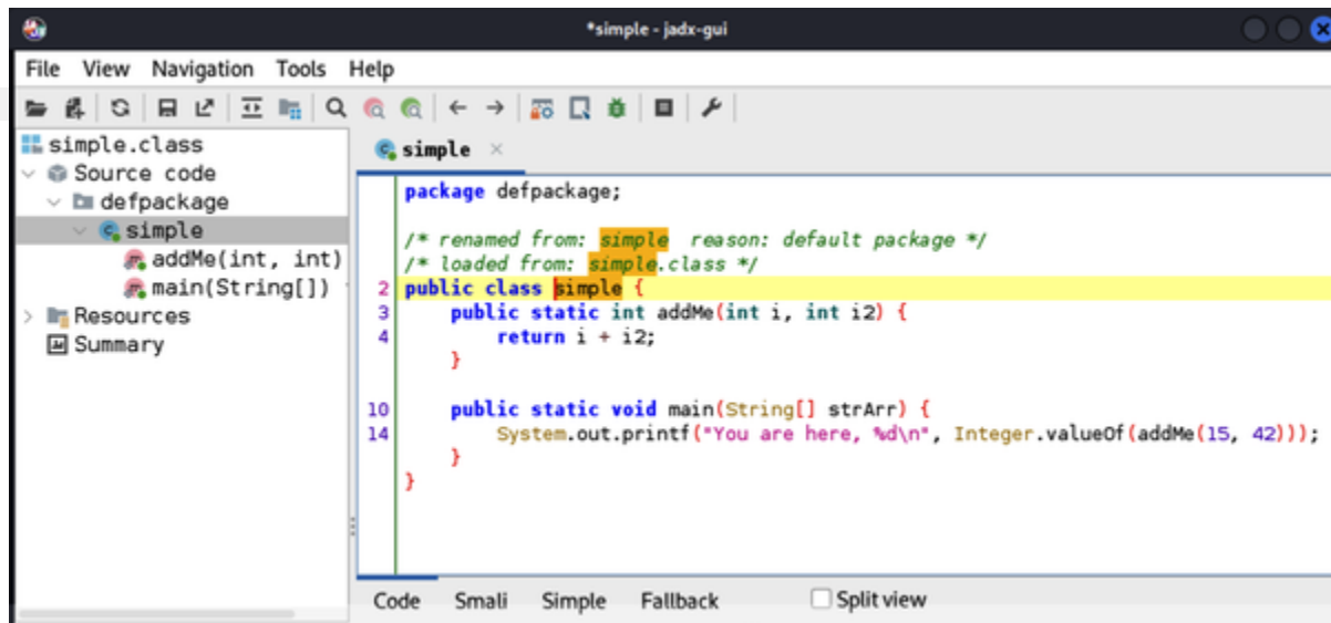
Figure 11-4. jadx-gui decompiler
