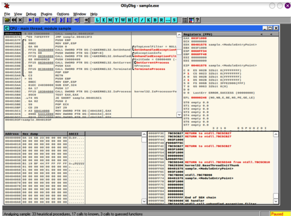
Figure 11-3. Ollydbg disassembler
