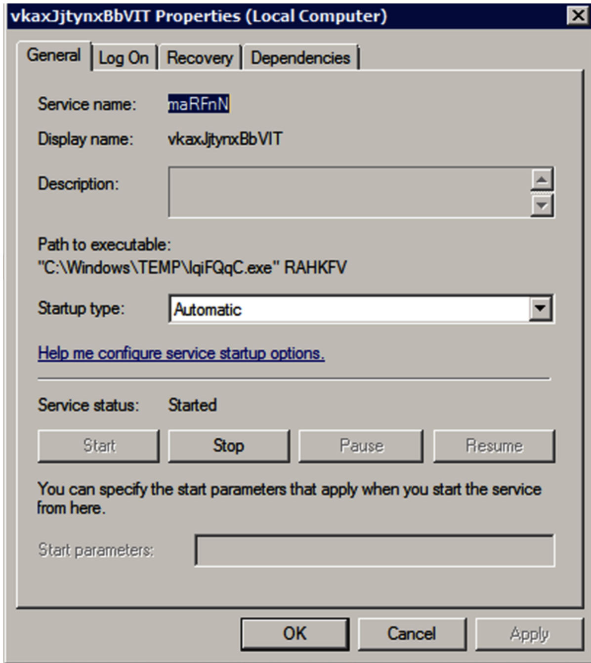
Figure 6-1. Service details
