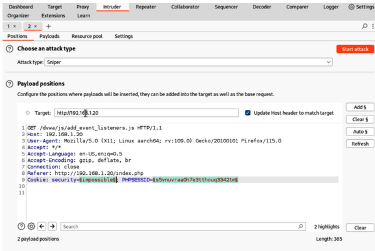
Figure 8-5. Burp Suite Intruder
