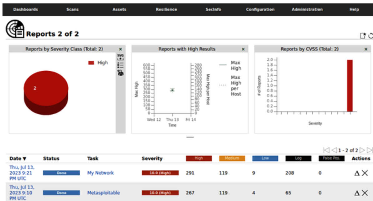
Figure 4-13. Report dashboard
