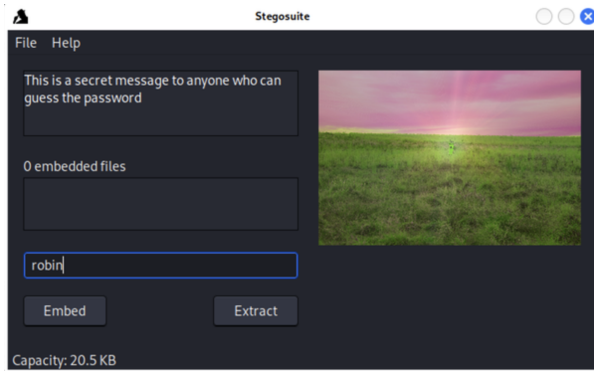
Figure 12-9. stegosuite GUI
