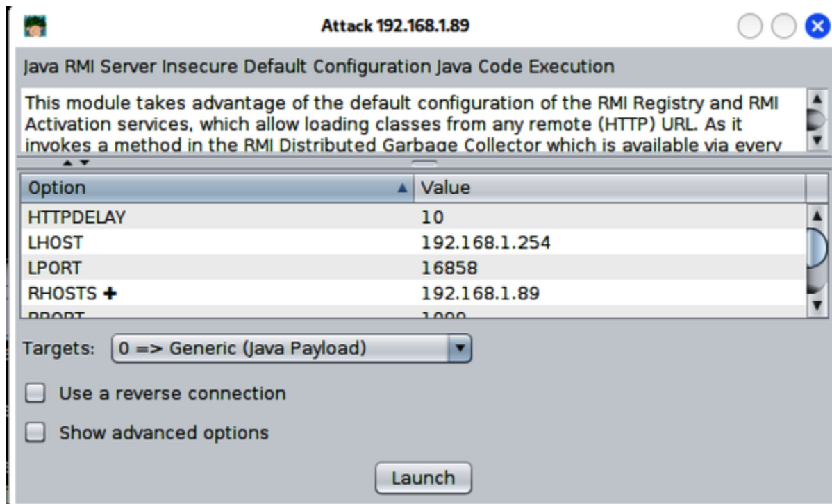
Figure 5-2. Exploit launch in Armitage
