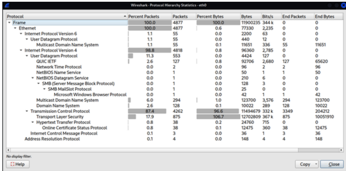
Figure 2-7. Protocol hierarchy in Wireshark
