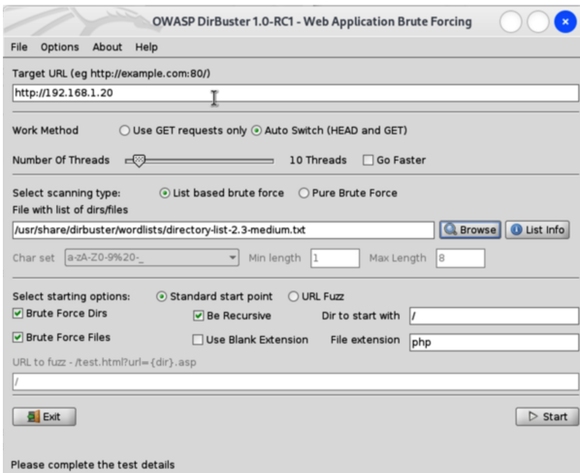
Figure 8-15. dirbuster testing a website
