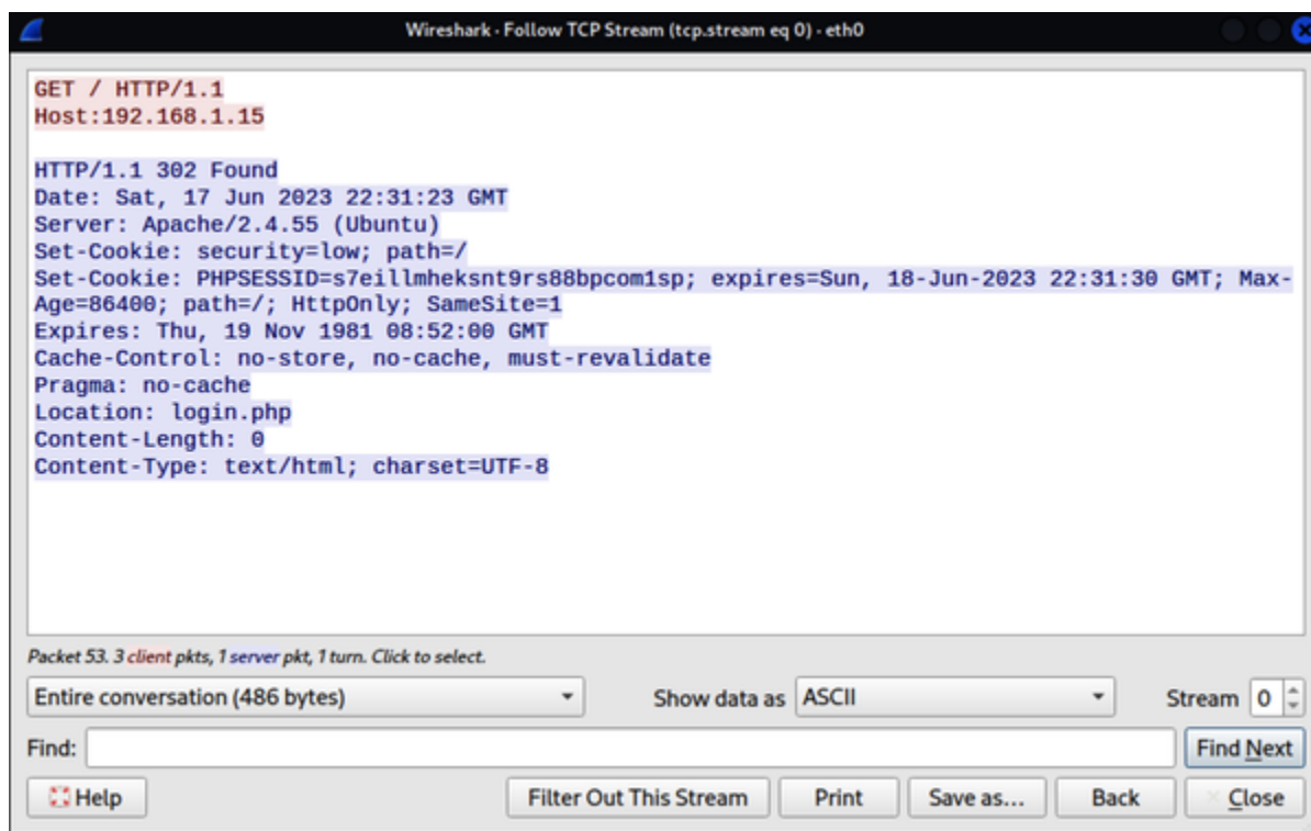
Figure 2-5. Following the TCP stream output
