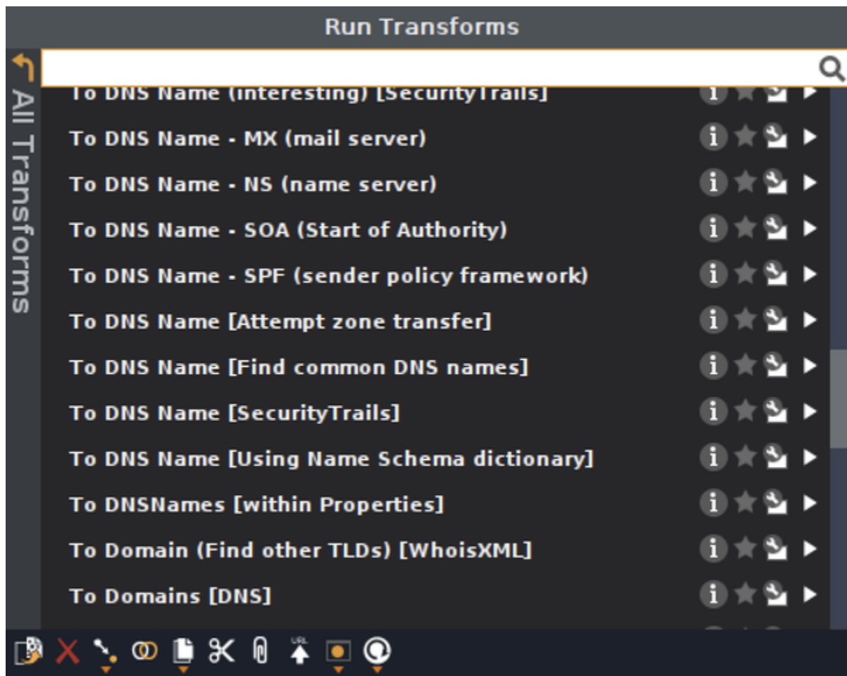
Figure 3-5. Transforms to apply to entities
