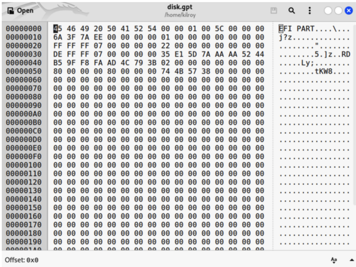
Figure 12-2. Hex representation of a GPT header block
