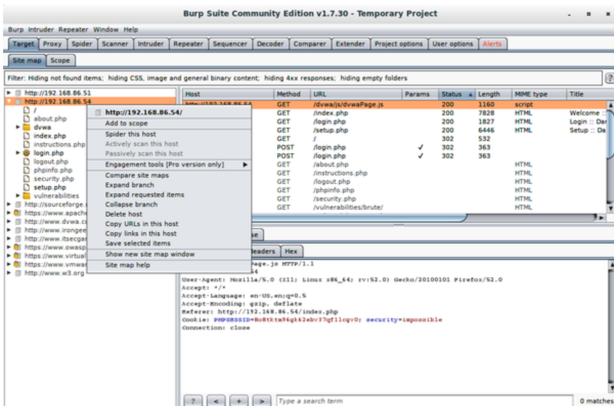
Figure 8-4. Burp Suite Target tab with spider
