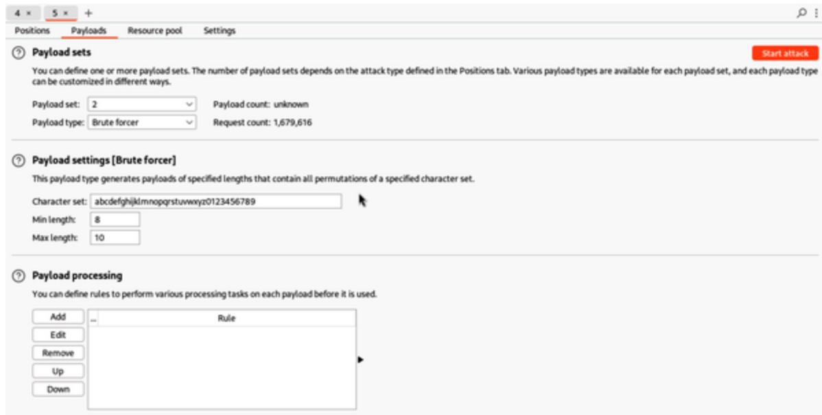
Figure 9-4. Brute-forcing usernames and passwords in Burp Suite
