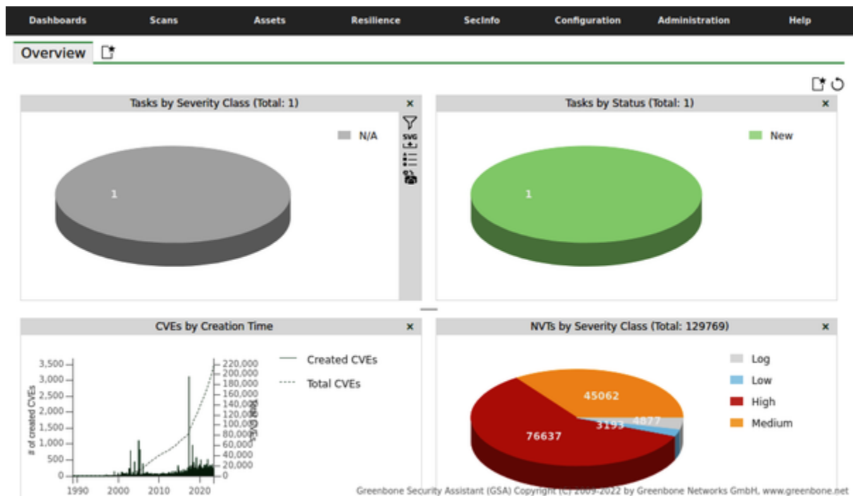
Figure 4-6. Greenbone Security Assistant
