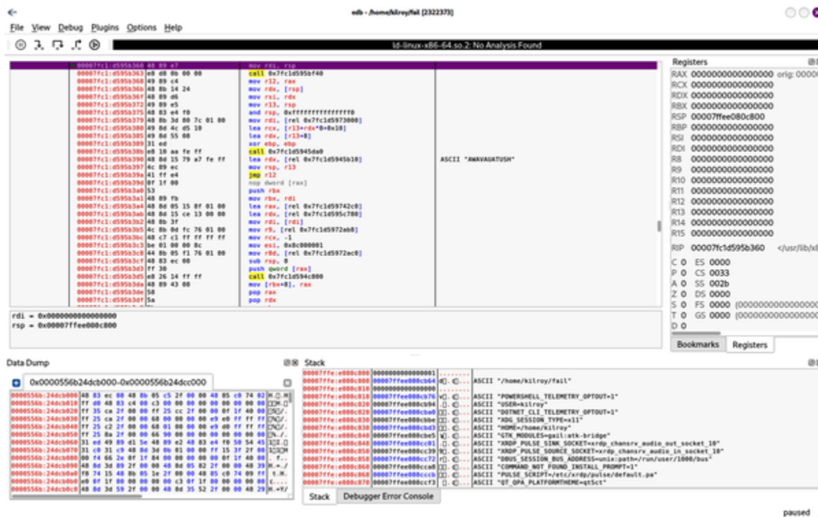
Figure 11-2. Disassembly with edb
