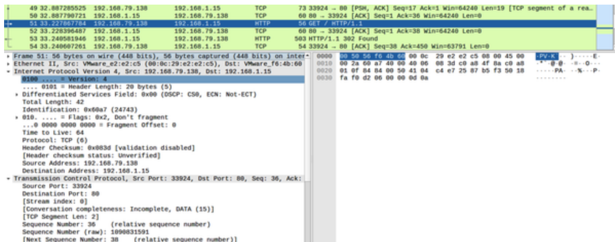
Figure 2-4. Header fields in Wireshark
