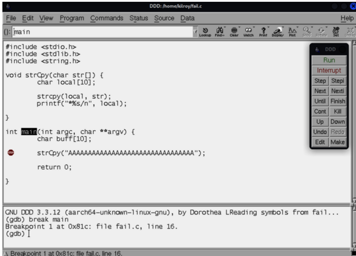
Figure 11-1. Debugging with ddd
