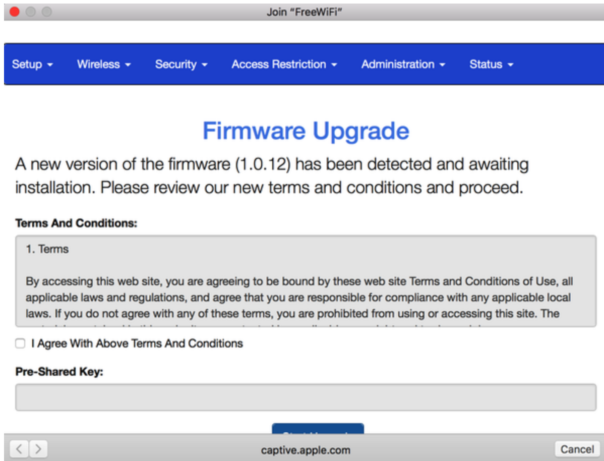
Figure 7-10. Captive login page from wifiphisher
