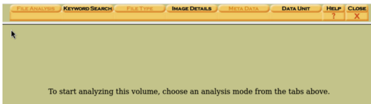
Figure 12-6. Autopsy menu
