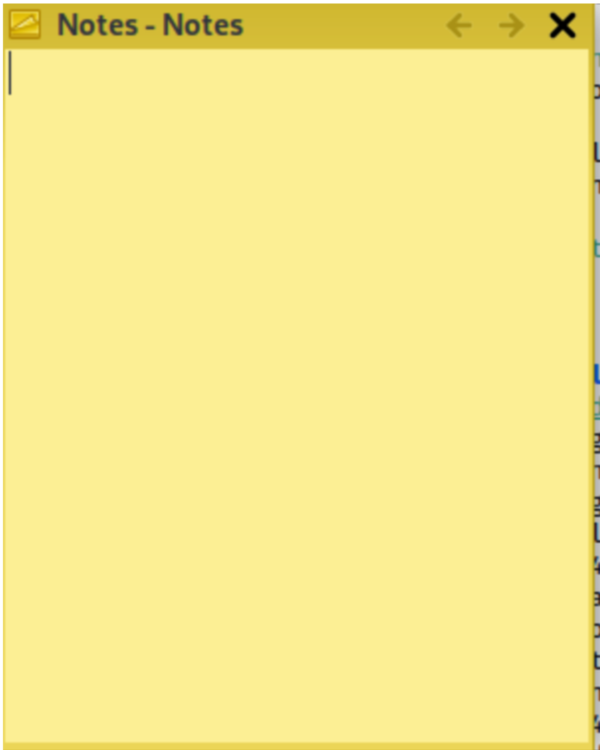
Figure 13-3. Notes application
