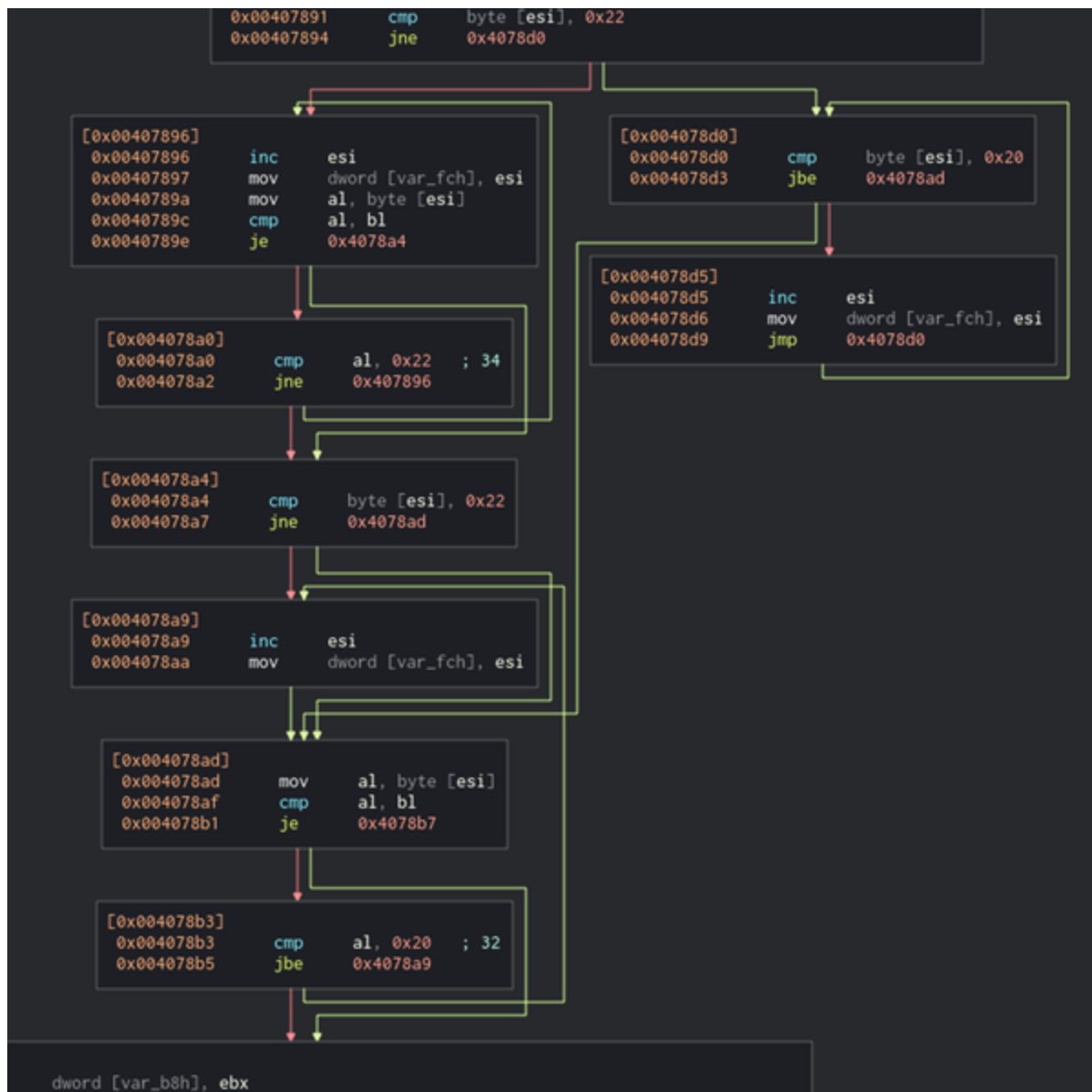
Figure 11-7. Graph of program in Cutter
