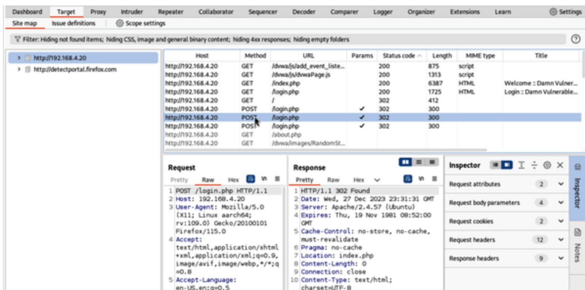
Figure 9-3. Burp Suite target selection
