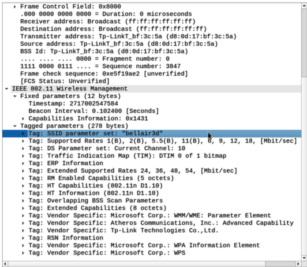
Figure 7-2. Radio headers in Wireshark
