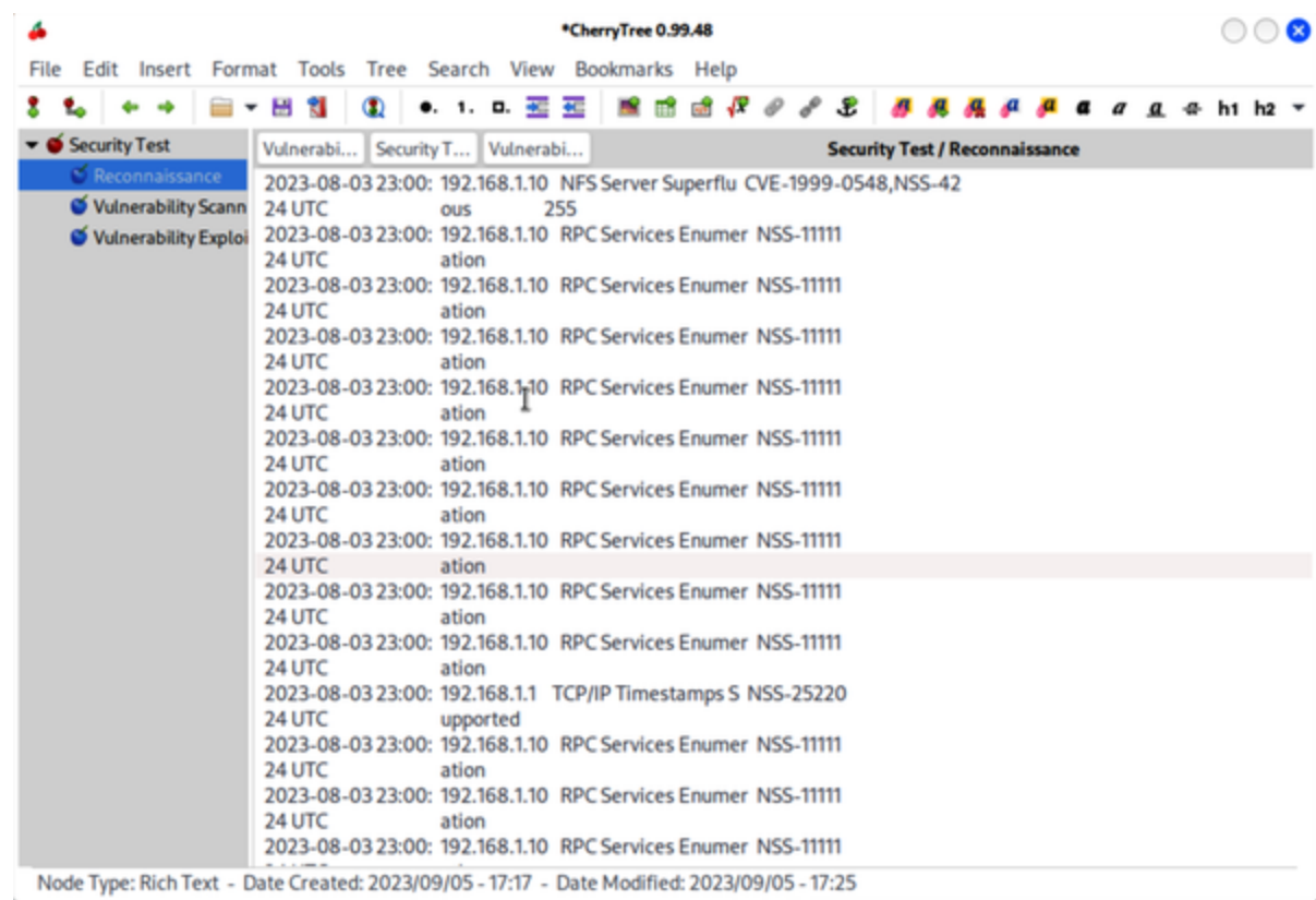
Figure 13-4. Cherry Tree notes organizer
