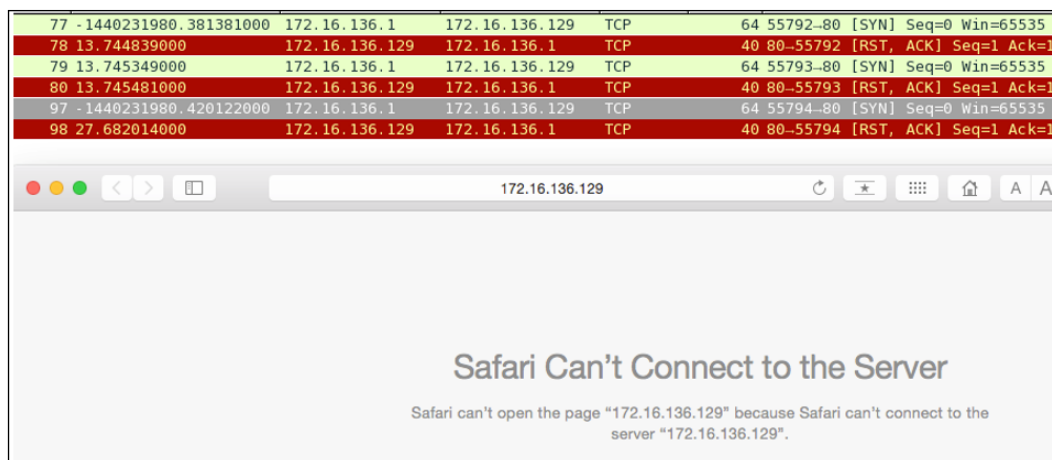
Figure 5.2: RST packets captured
