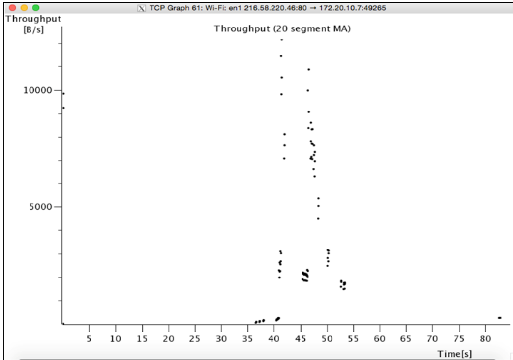
Figure 3.15: Throughput Graph
