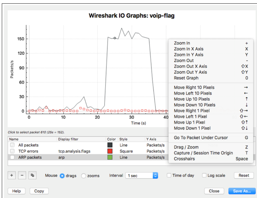
Figure 9.14: The right-click options list
