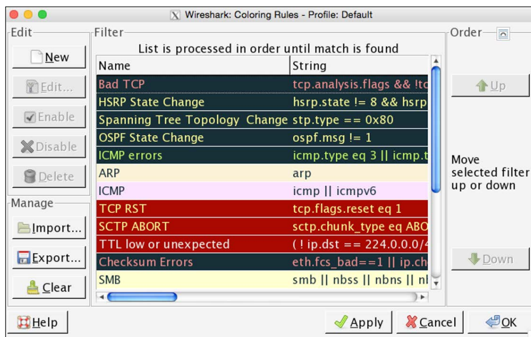
Figure 2.16: Coloring rules
