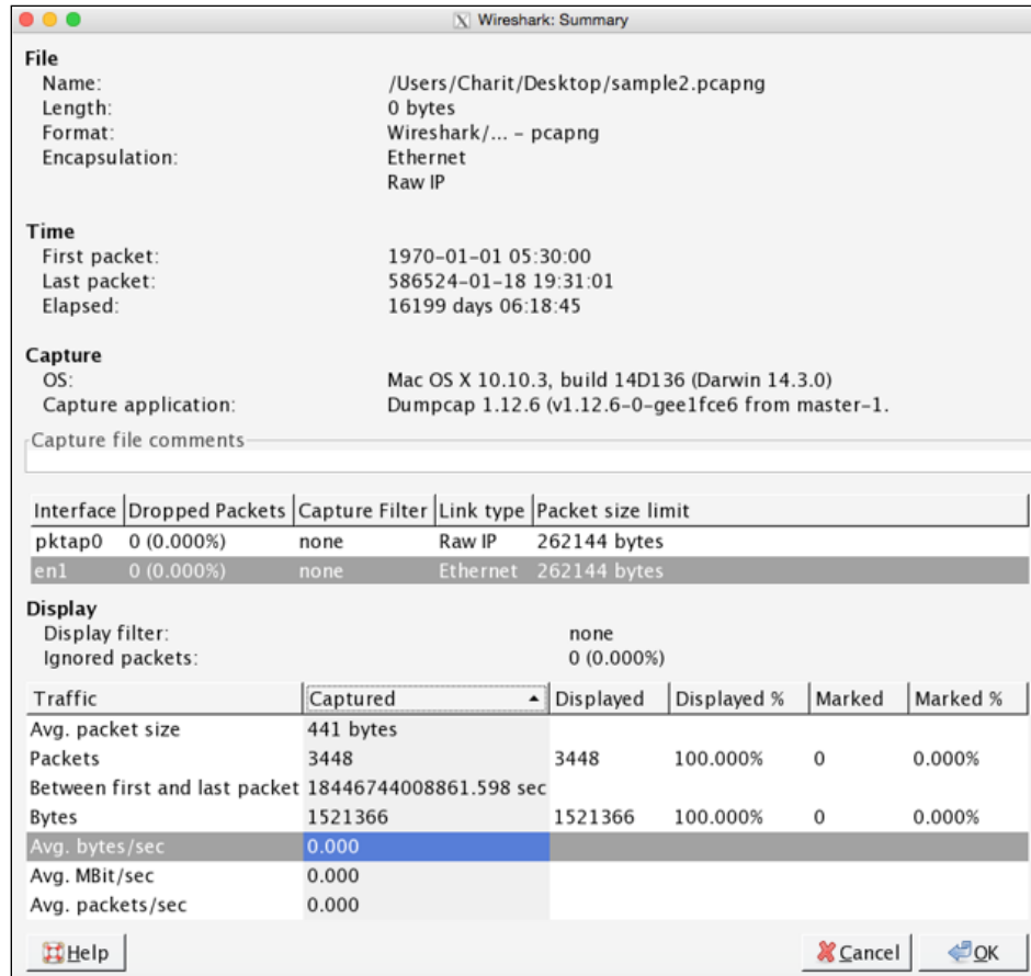
Figure 3.1: Summary dialog
