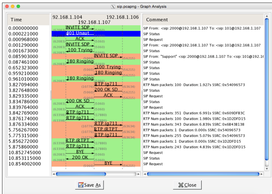
Figure 4.24: Flow graph
