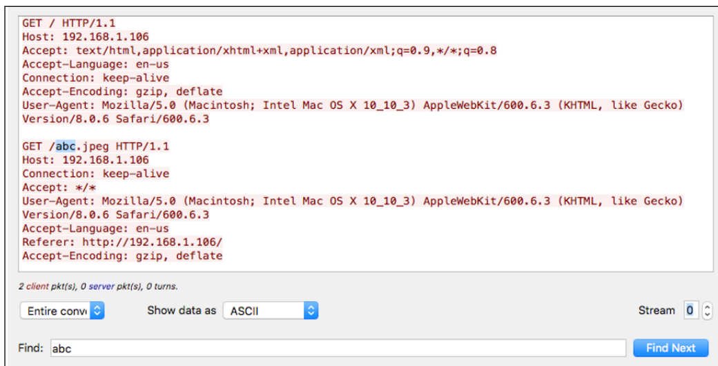
Figure 9.22: The Find utility in the Follow TCP stream dialog
