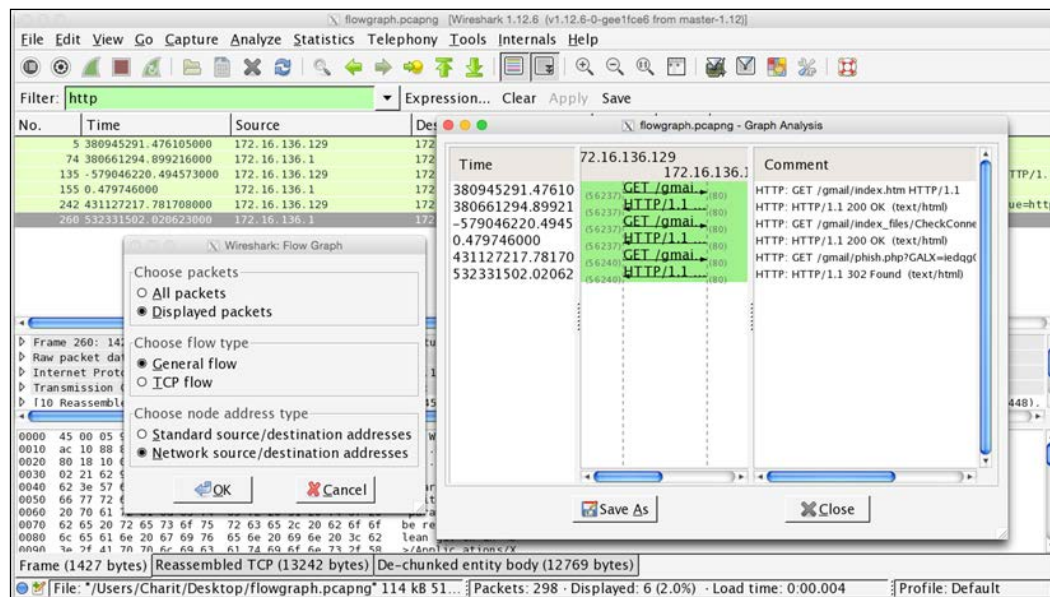
Figure 3.13: Flowgraph
