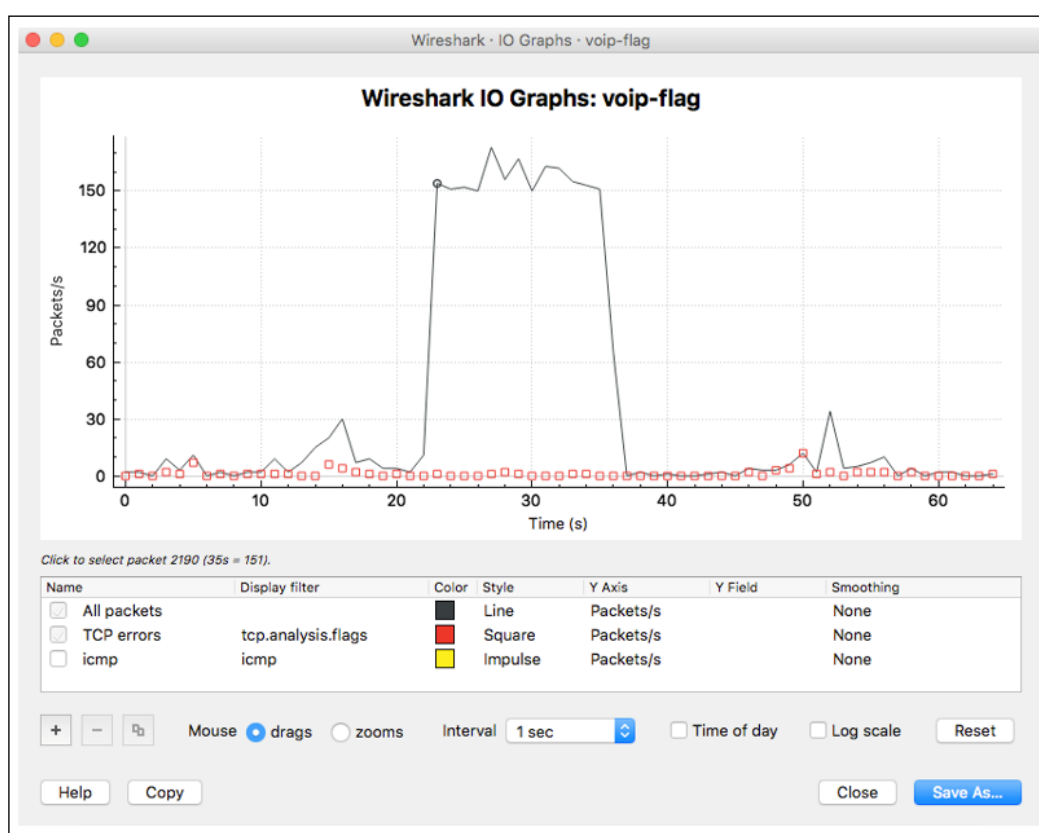
Figure 9.11: The IO graph
