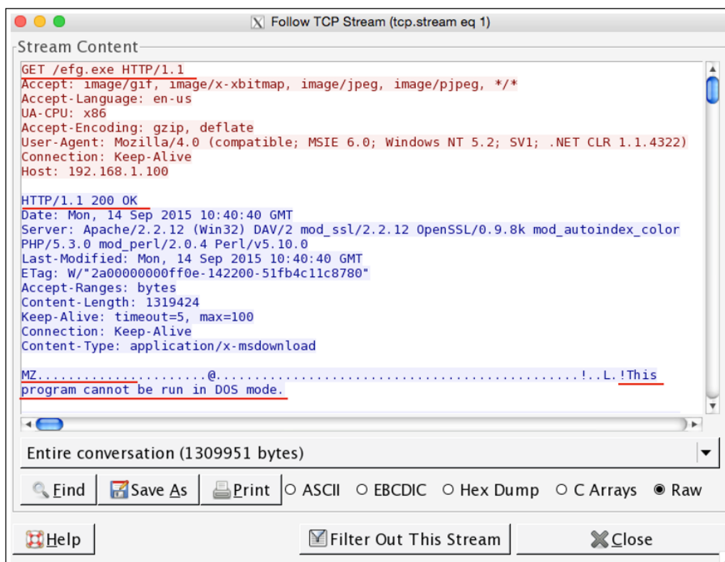
Figure 7.22: Malware signature
