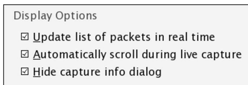
Figure 2.7: Display Options
