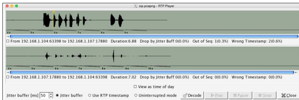
Figure 4.27: RTP Player
