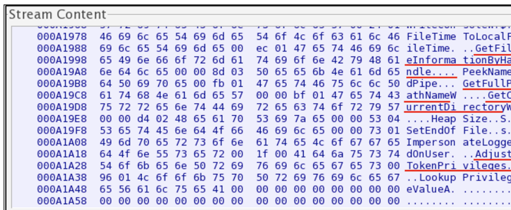
Figure 7.26: Hexdump in TCP stream dialog
