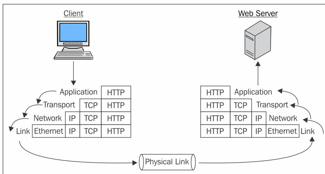
Figure 1.1: Data encapsulation
