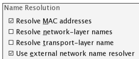
Figure 2.8: Name Resolution
