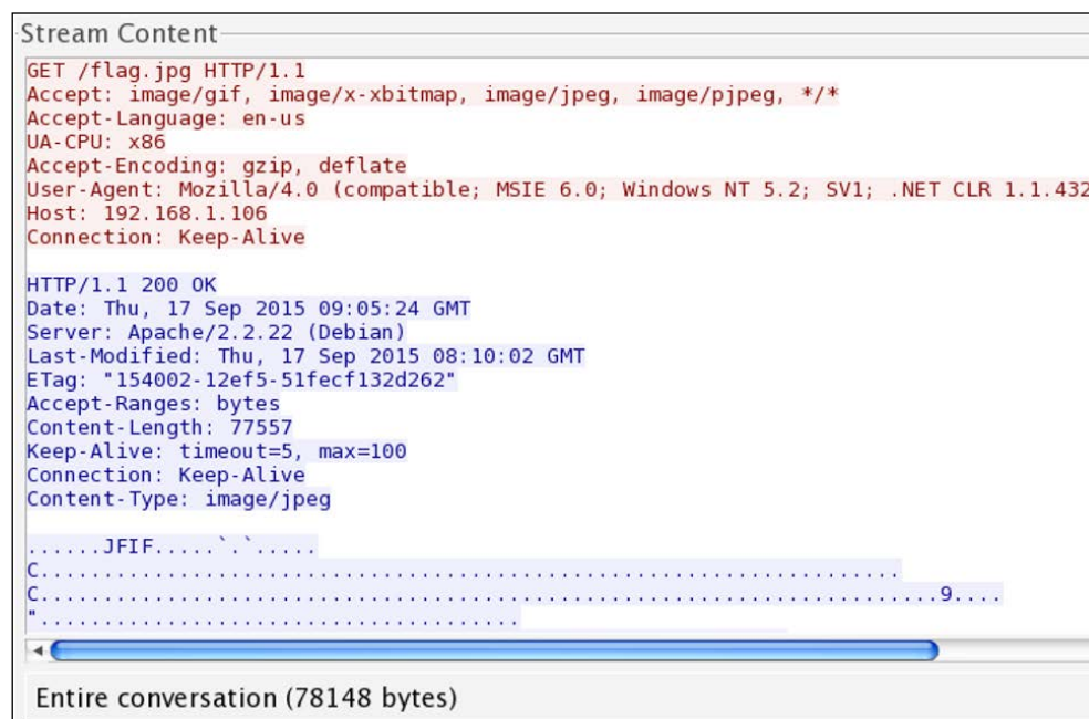
Figure 7.35: TCP stream – CTF2
