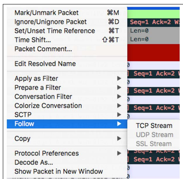
Figure 9.18: Follow TCP streams
