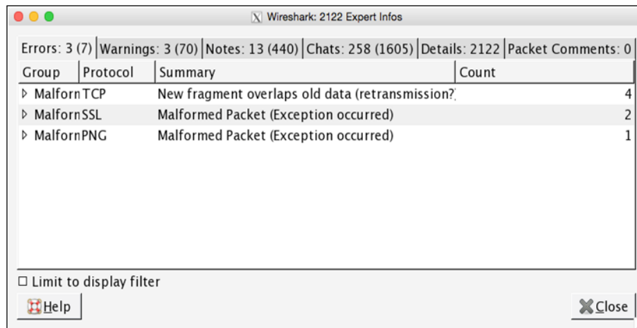
Figure 3.19: Expert Infos dialog
