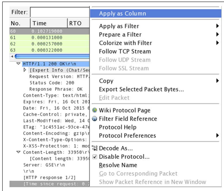
Figure 8.14: Apply Time since request as a column
