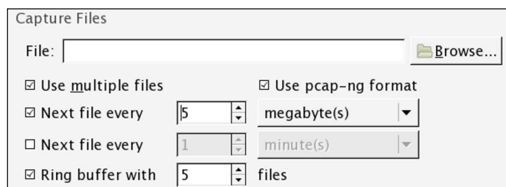
Figure 2.5 : The Capture Files option
