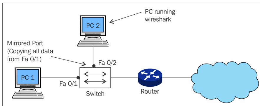
Figure 1.2: Port mirroring
