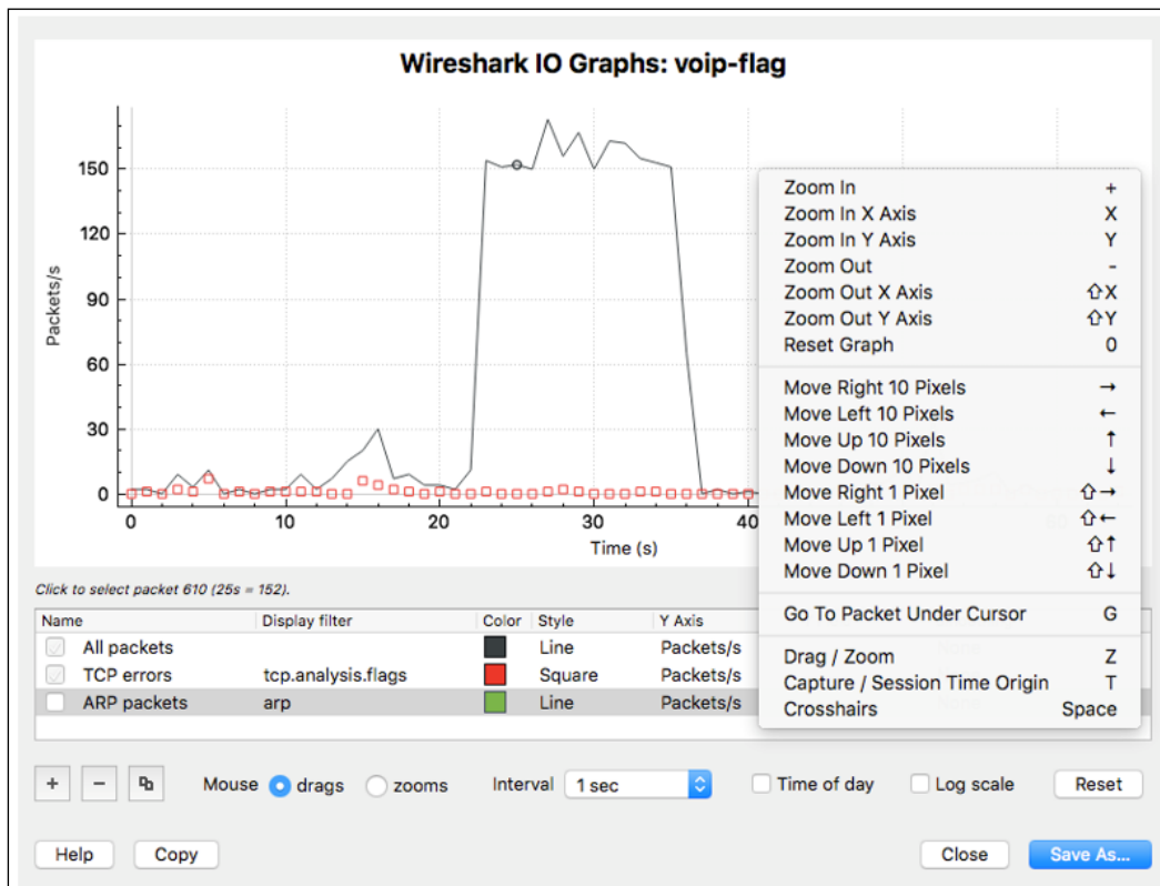
Figure 9.15: Comparing two graphs at a single instance
