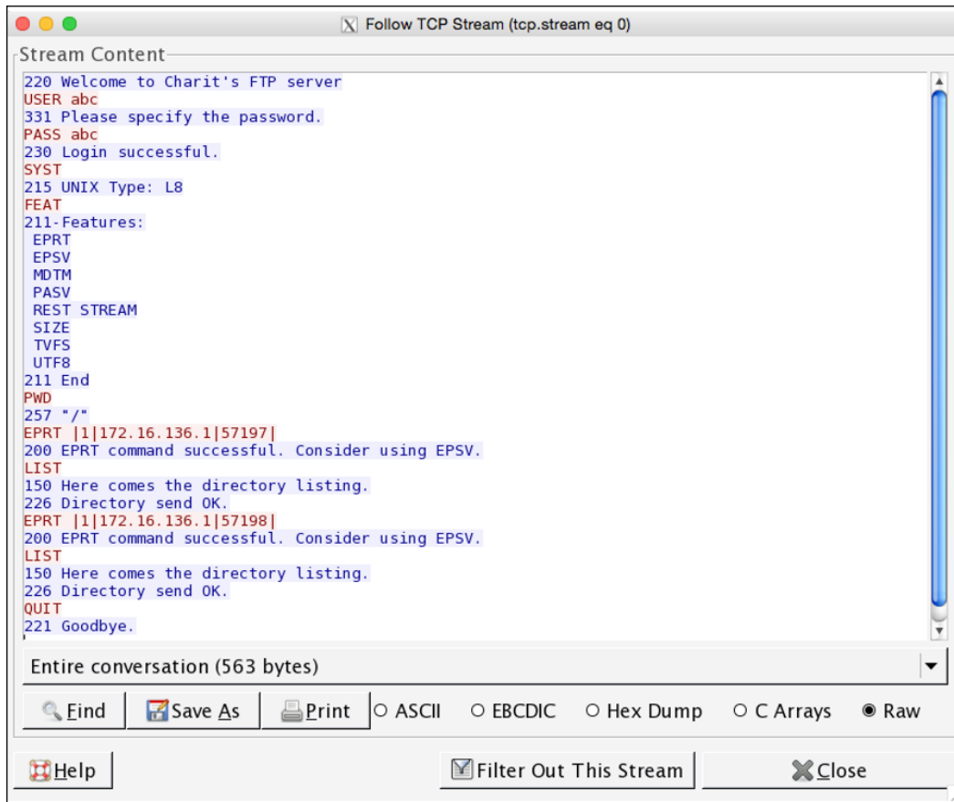
Figure 4.10: FTP stream
