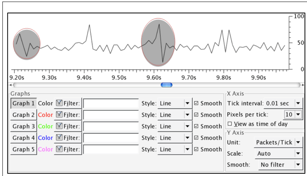
Figure 8.23: A bottleneck scenario
