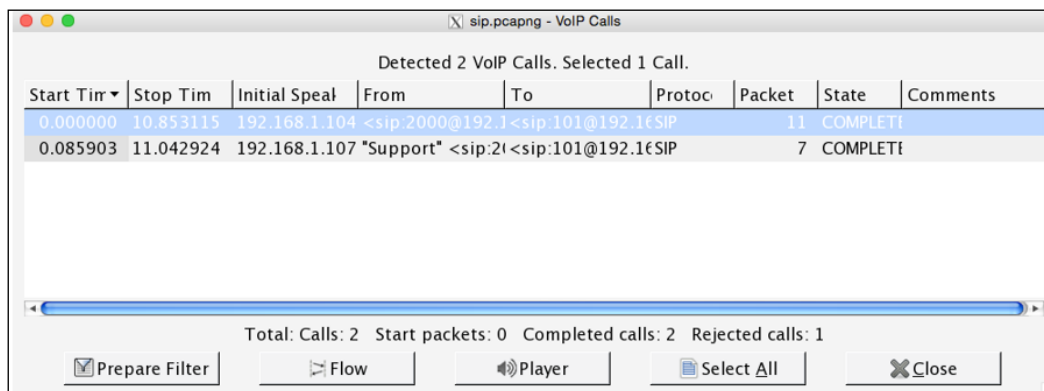
Figure 4.25 : VOIP Calls dialog
