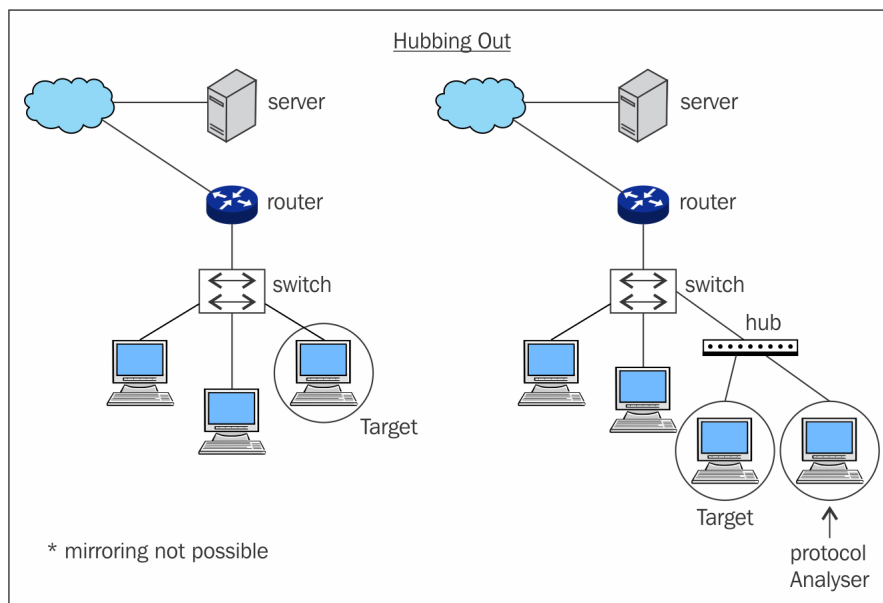
Figure 1.3: Hubbing out
