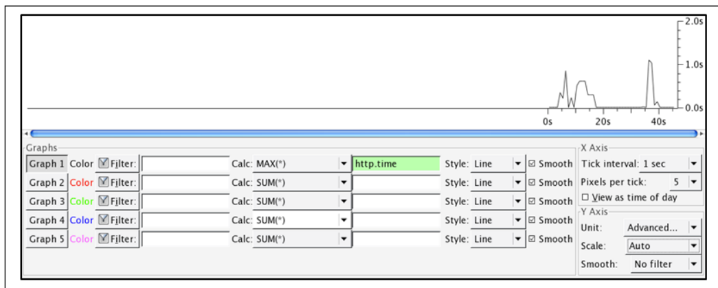
Figure 8.17: Using an IO graph to identify the delays in HTTP response
