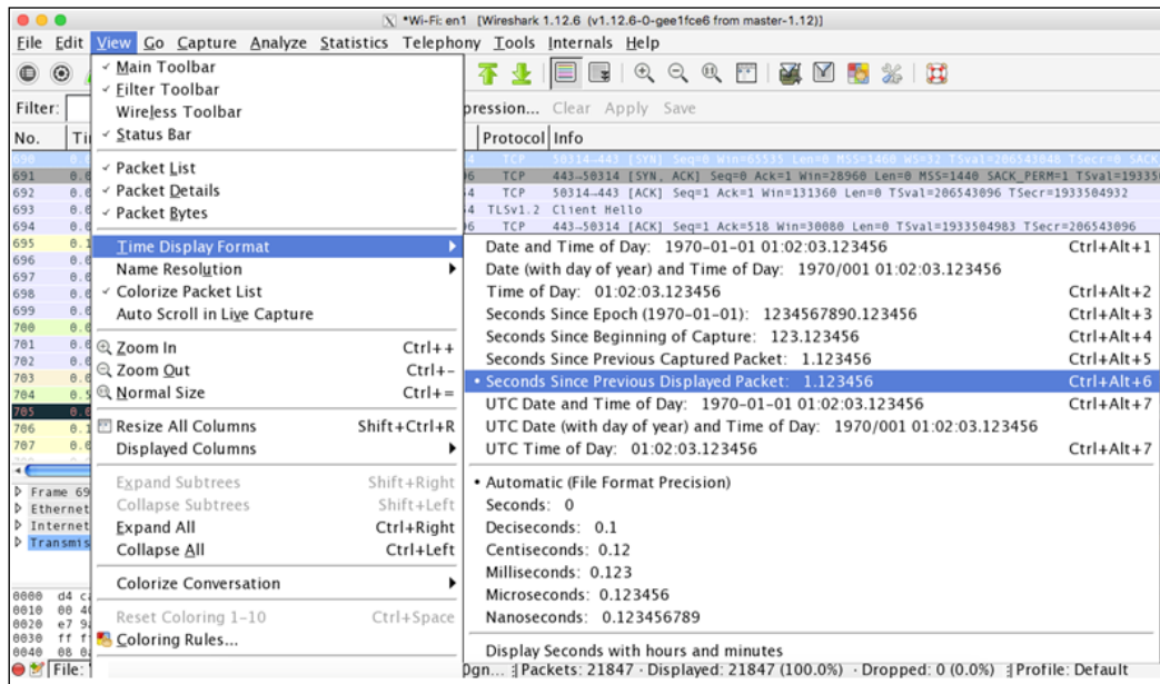
Figure 8.7: Customizing the time column
