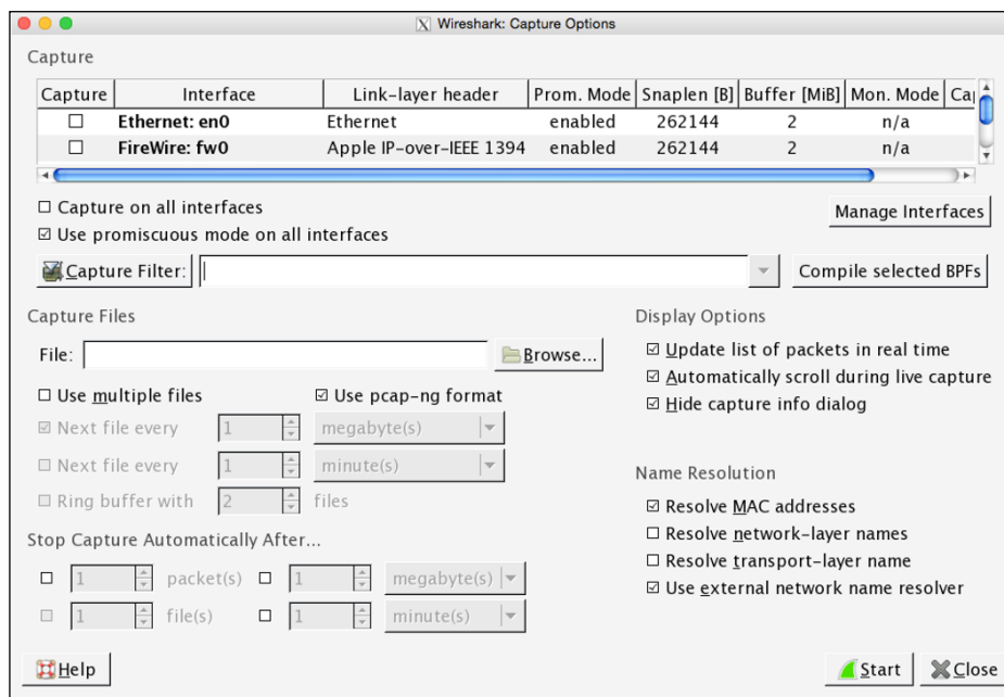
Figure 2.1: The Capture Options dialog
