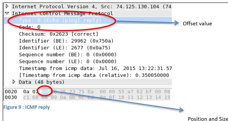
Figure 2.9: ICMP reply
