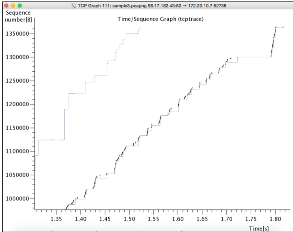
Figure 3.16 : Time Sequence graph (tcptrace)
