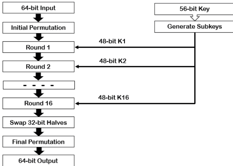
Figure 4.5 – The DES encryption process
