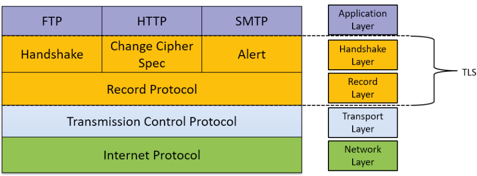
Figure 9.18 – The TLS protocol stack
