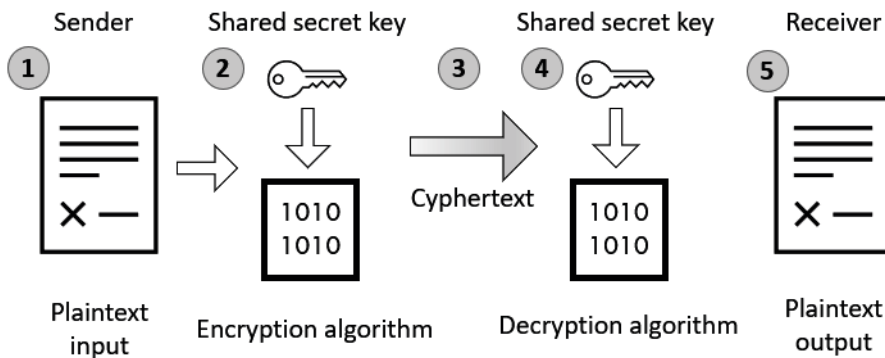
Figure 4.3 – Symmetric encryption process
