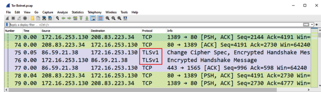
Figure 7.1 – TOR activity on a network
