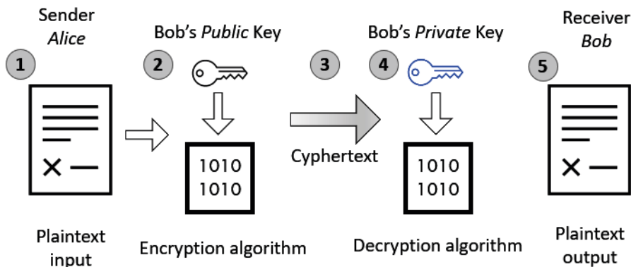
Figure 5.7 – Encrypting mail using PGP
