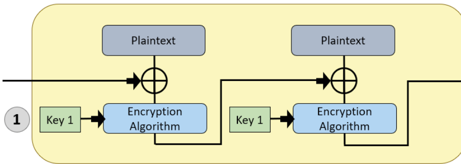
Figure 6.10 – CBC mode
