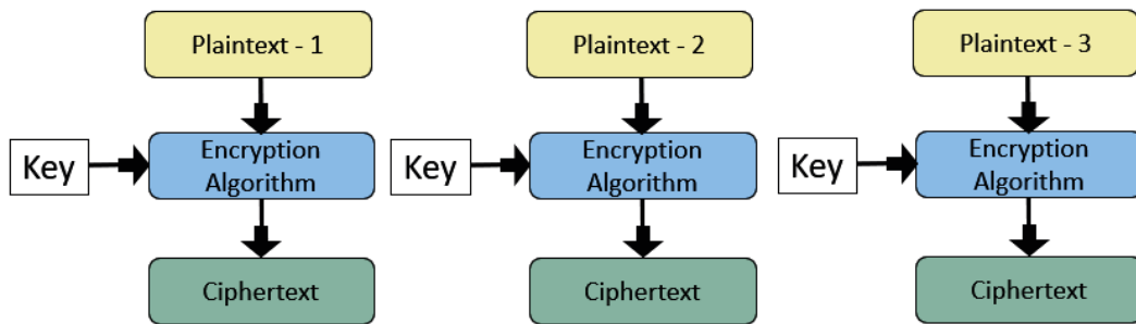
Figure 4.12 – ECB
