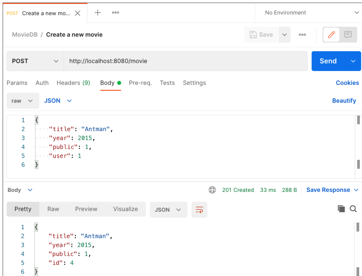
Figure 10.5 Creating a New Data Record with Postman
