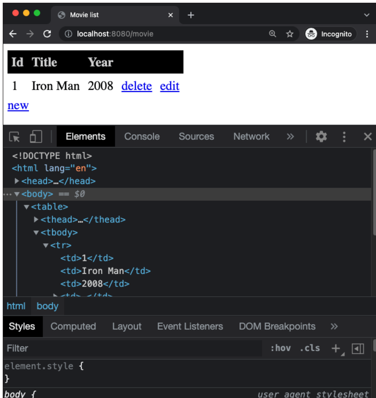
Figure 7.2 HTML Source Code of the List Display
