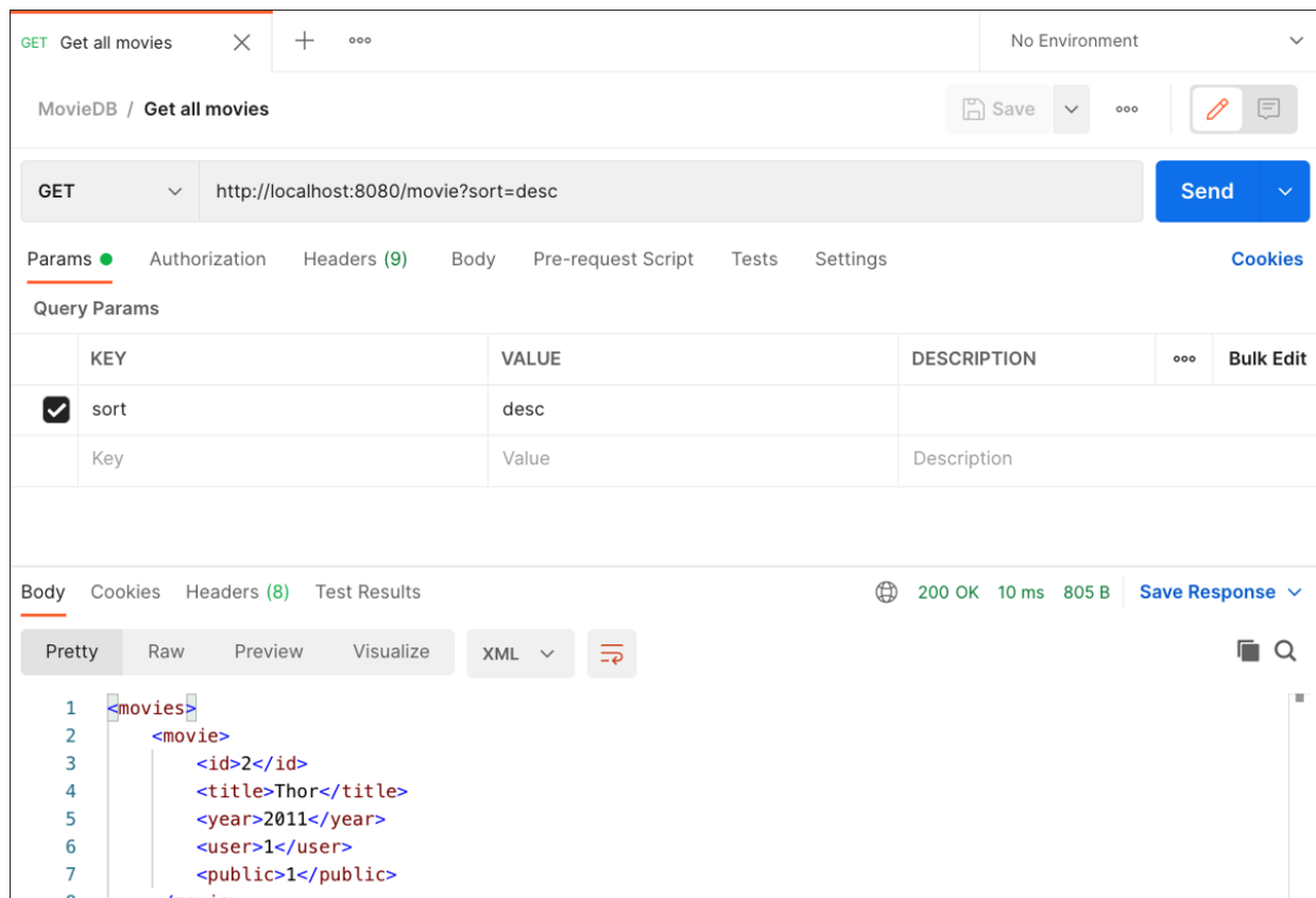
Figure 10.4 Sorting the Movie List with Postman
