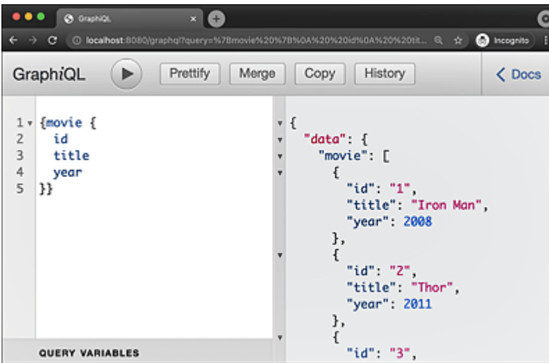
Figure 11.2 GraphQL Query of the Data from the Database
