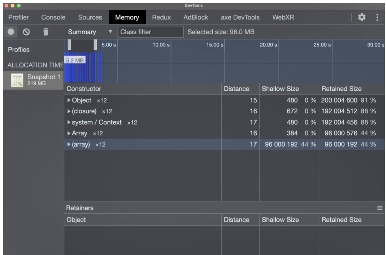
Figure 26.6 Recording Memory Consumption over Time
