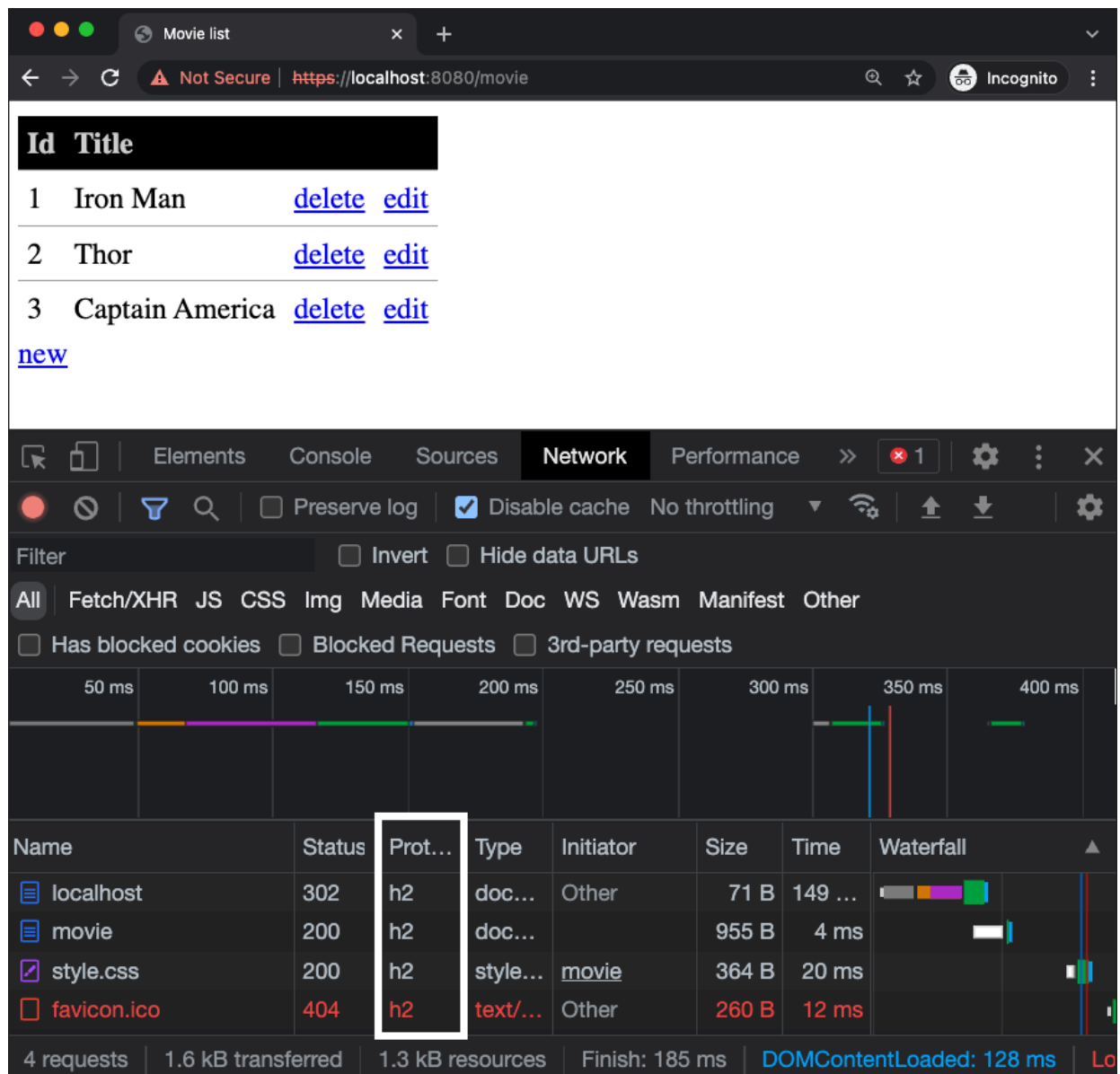
Figure 6.10 Delivery of Resources via the h2 Protocol
