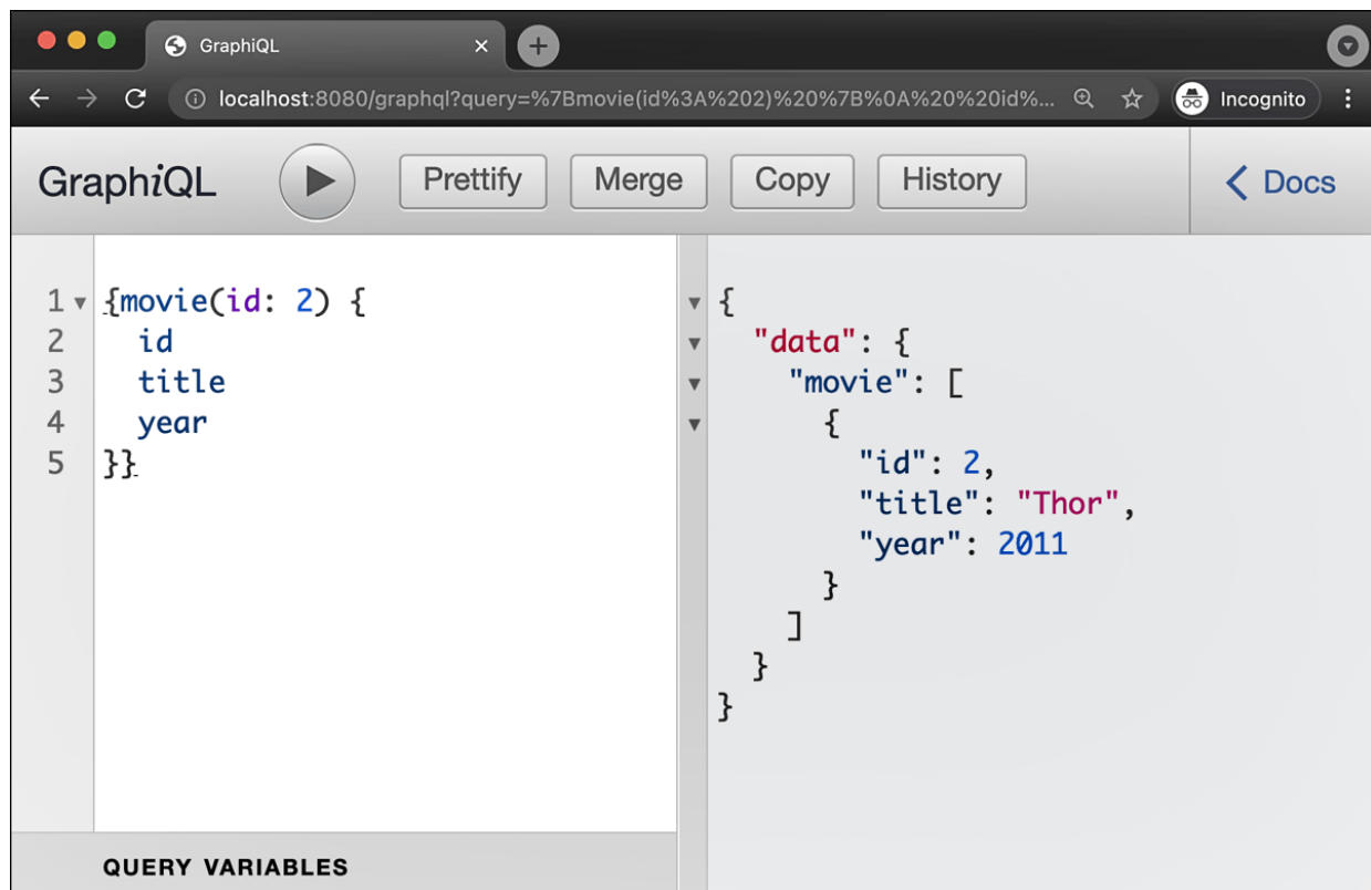
Figure 11.3 Querying a Data Record with GraphiQL
