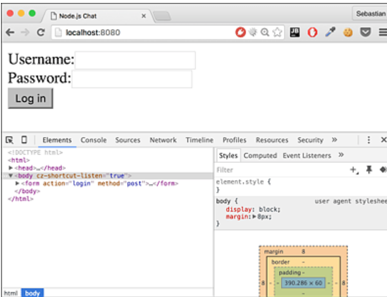
Figure 12.1 Login Screen
