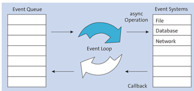
Figure 1.4 Event Loop
