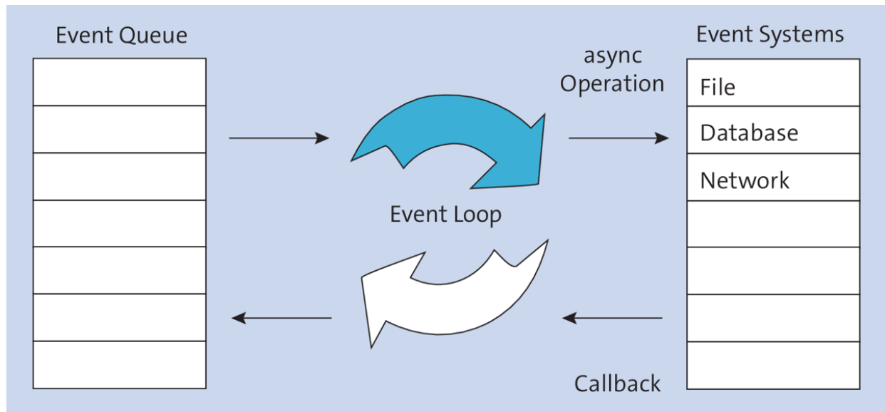
Figure 1.4 Event Loop
