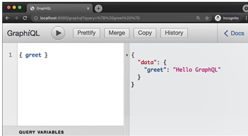
Figure 11.1 GraphQL View
