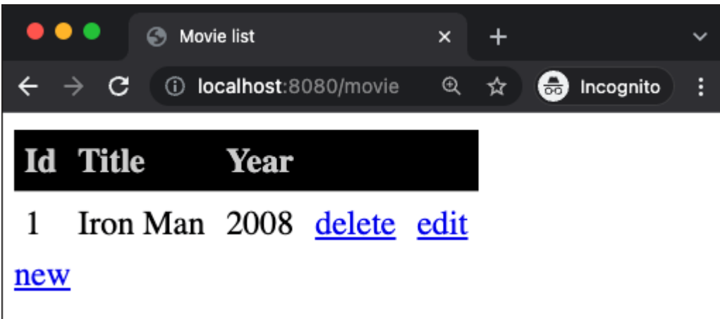
Figure 7.1 List View
