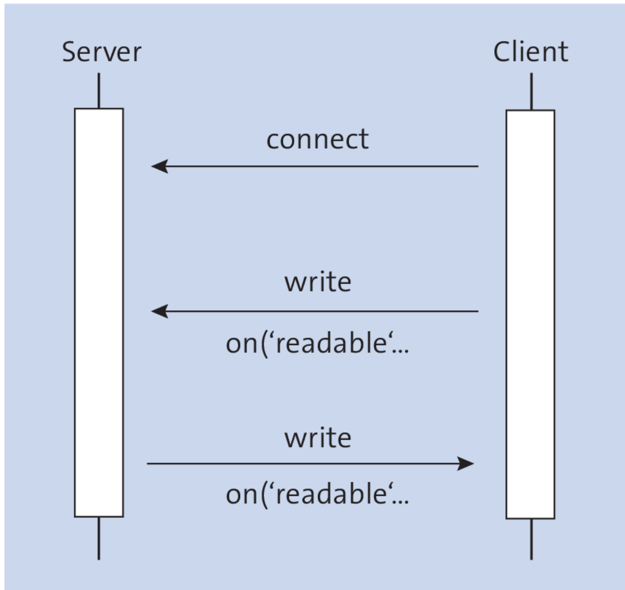
Figure 20.2 Socket Communication
