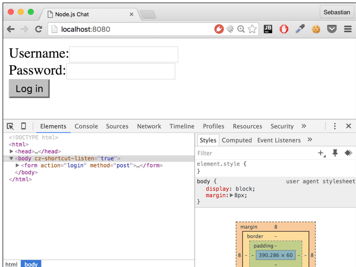
Figure 12.1 Login Screen
