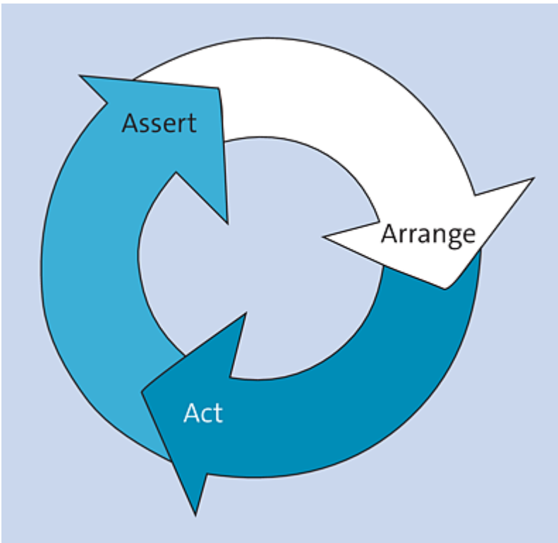
Figure 23.1 AAA Process
