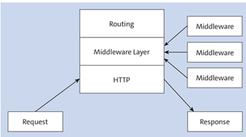
Figure 6.1 Express Structure
