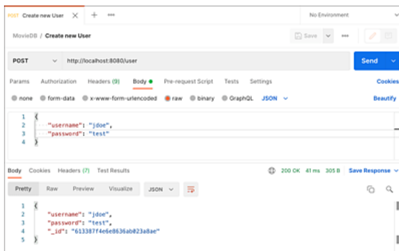
Figure 27.6 Creating a New User with Postman
