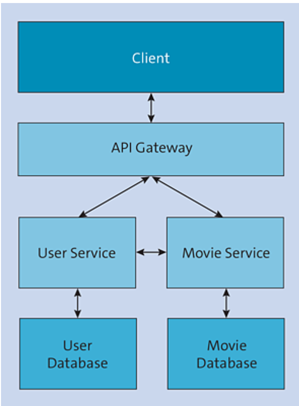
Figure 27.8 Movie Service in the Microservice Architecture
