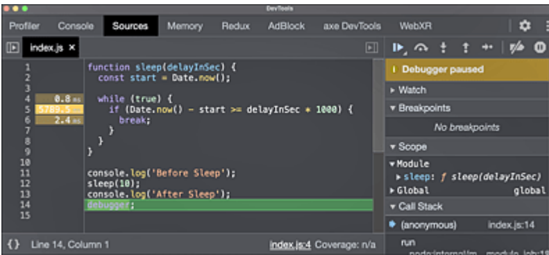
Figure 26.3 Display of Execution Time in DevTools
