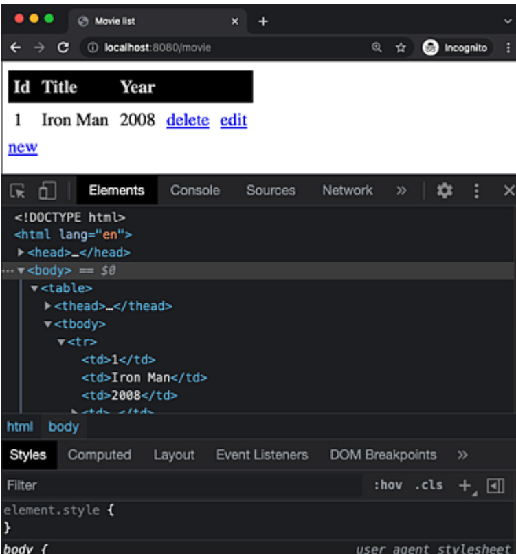
Figure 7.2 HTML Source Code of the List Display
