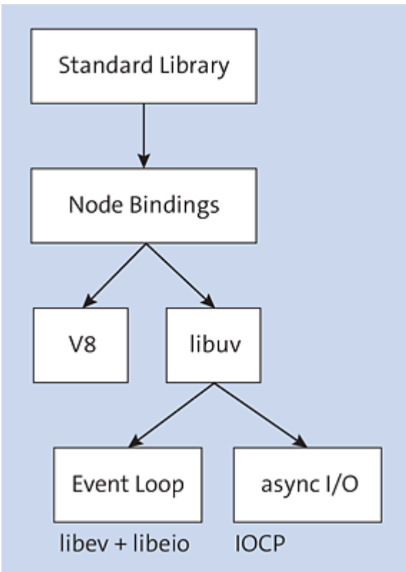
Figure 4.1 Structure of Node.js
