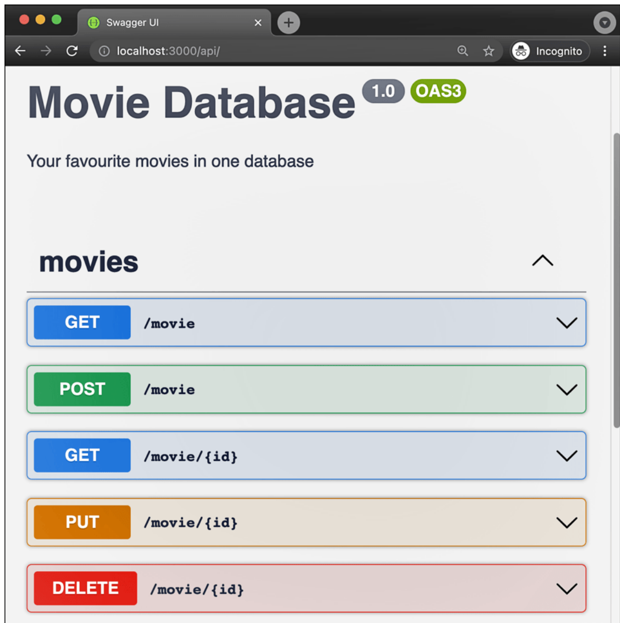
Figure 14.3 API Documentation of the MovieDB Application
