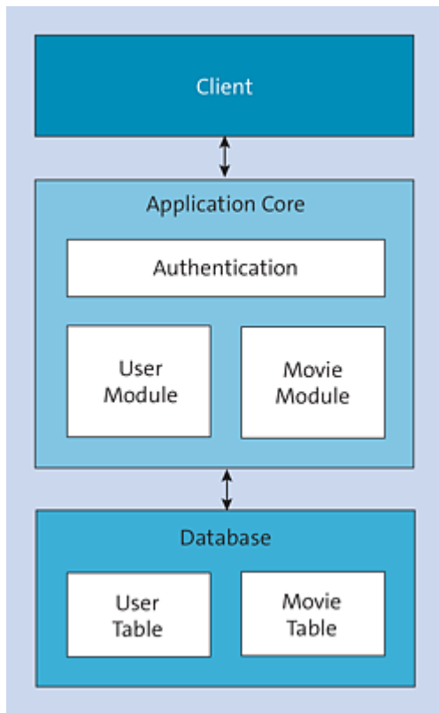
Figure 27.1 Monolithic Architecture
