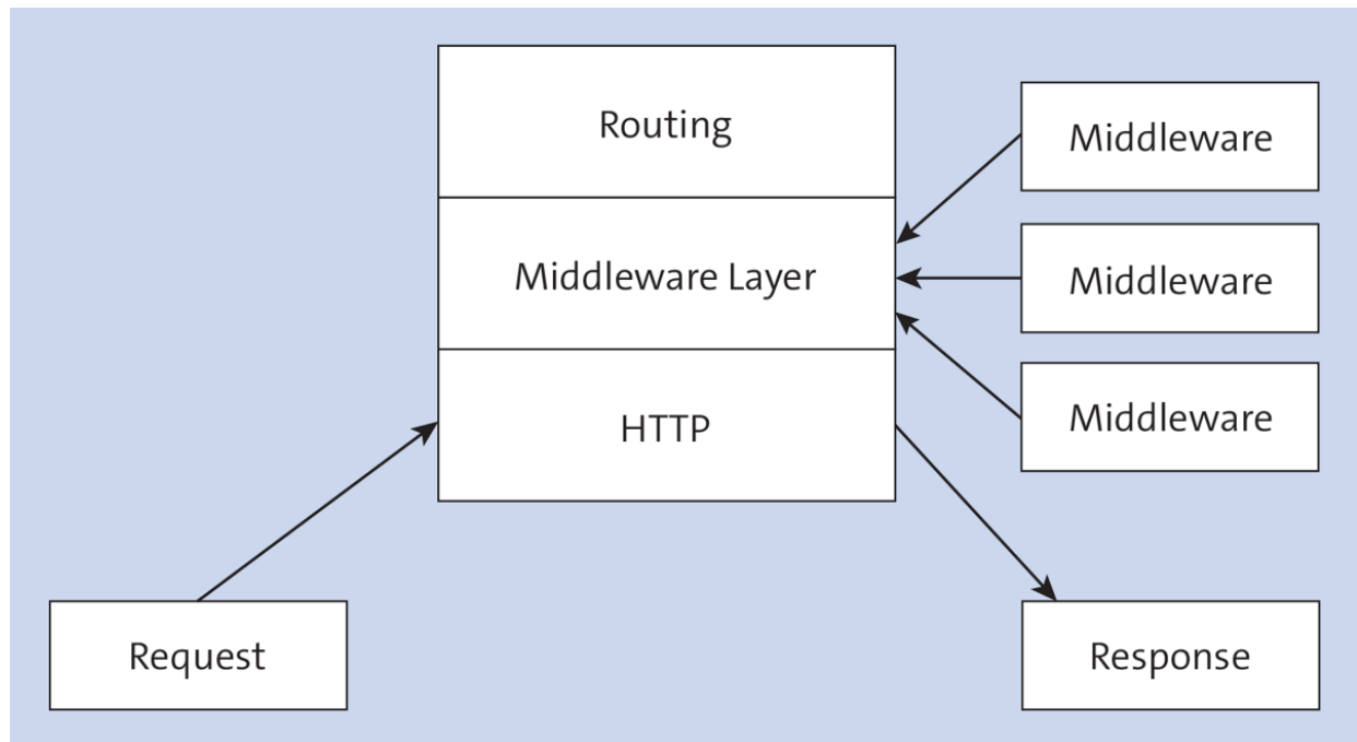
Figure 6.1 Express Structure
