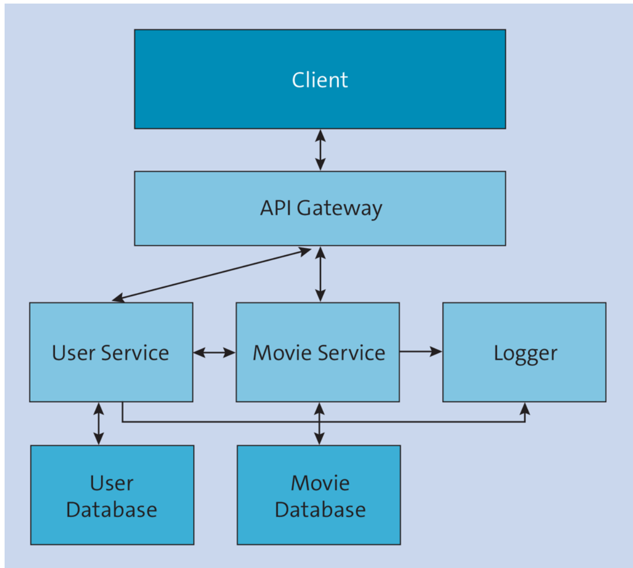
Figure 27.2 Microservice Architecture
