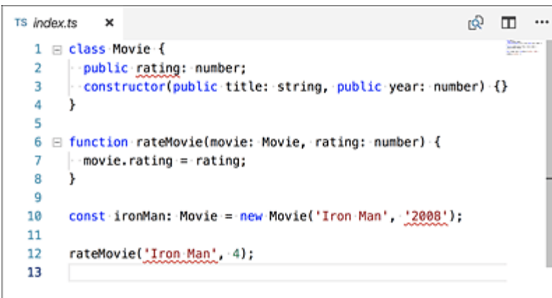
Figure 13.1 Error Messages with TypeScript in Visual Studio Code
