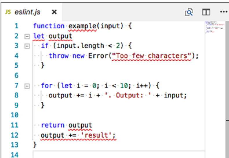
Figure 22.2 ESLint in Visual Studio Code
