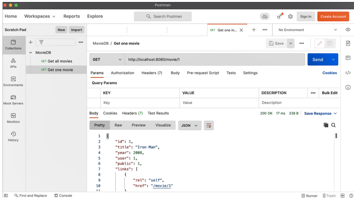
Figure 10.3 Querying a Data Record with Postman
