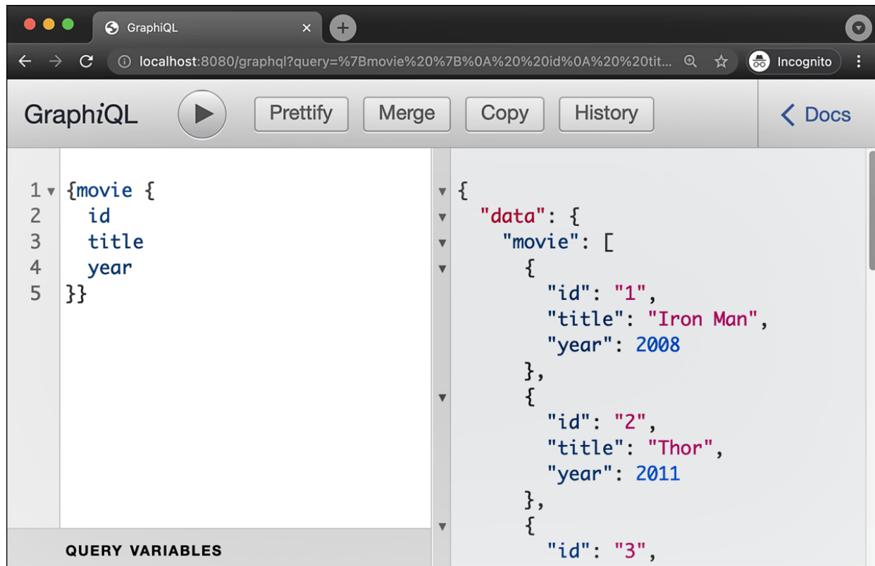
Figure 11.2 GraphQL Query of the Data from the Database
