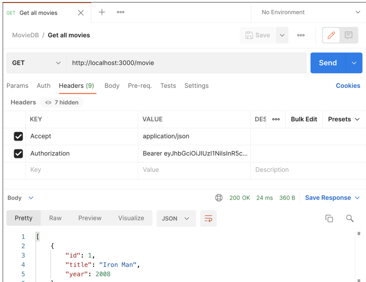
Figure 14.4 Request to the Movie Controller with a Valid Token
