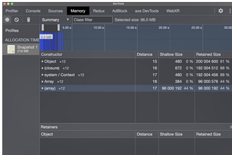
Figure 26.6 Recording Memory Consumption over Time
