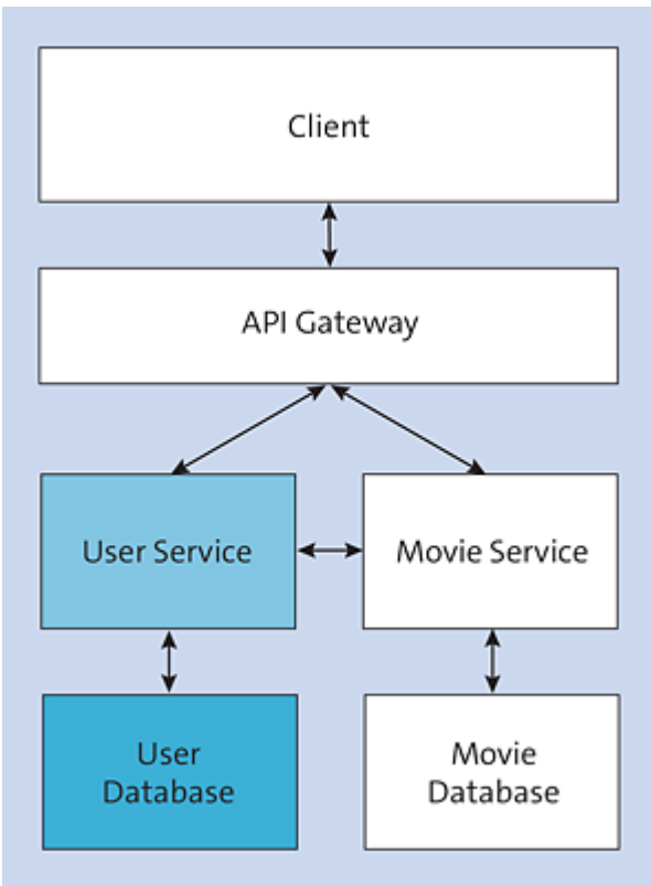
Figure 27.5 User Service in the Microservice Architecture
