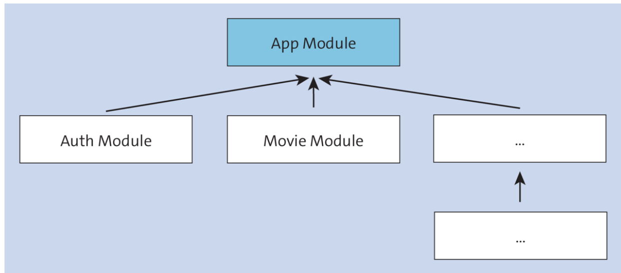
Figure 14.2 Modular Structure of a Nest Application
