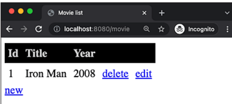
Figure 7.1 List View
