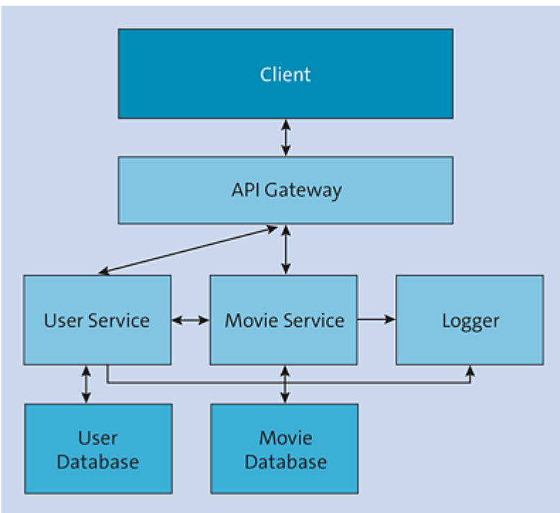
Figure 27.2 Microservice Architecture
