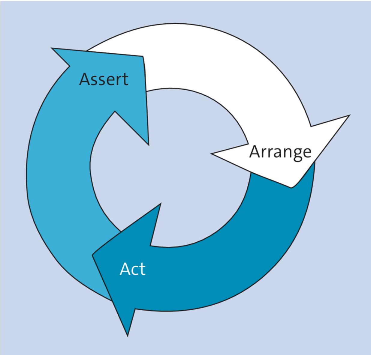
Figure 23.1 AAA Process
