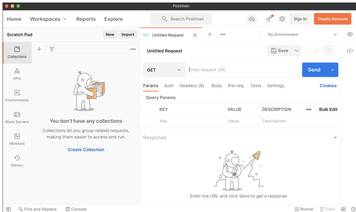
Figure 10.1 Postman GUI
