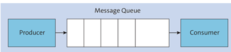
Figure 27.3 Message Queue
