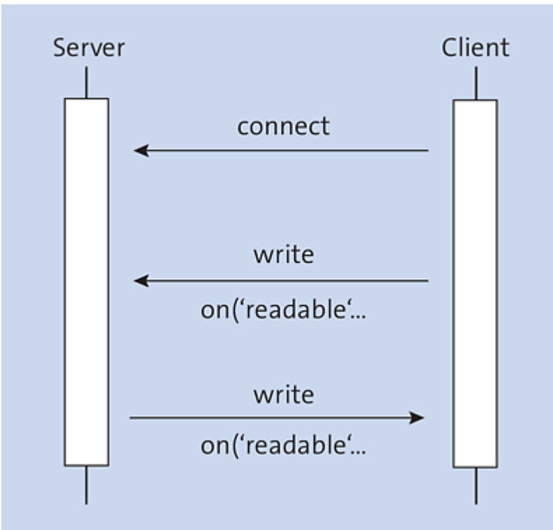
Figure 20.2 Socket Communication
