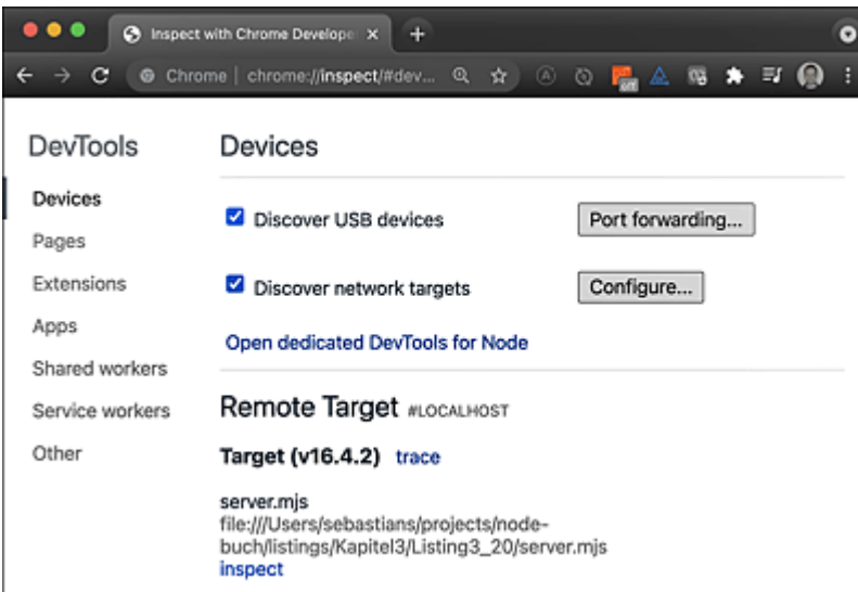
Figure 3.5 List of Debugging Sessions in Chrome
