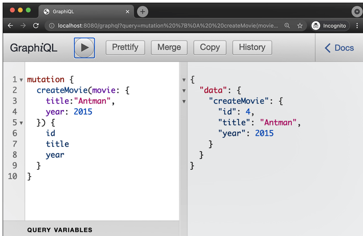
Figure 11.4 Creating a New Data Record
