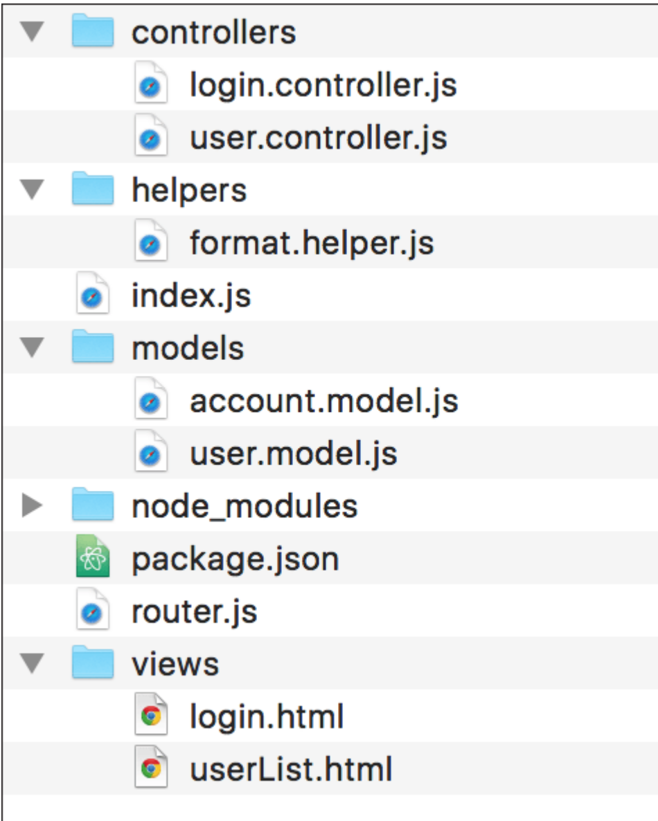
Figure 6.4 Structure for Medium-Size Applications
