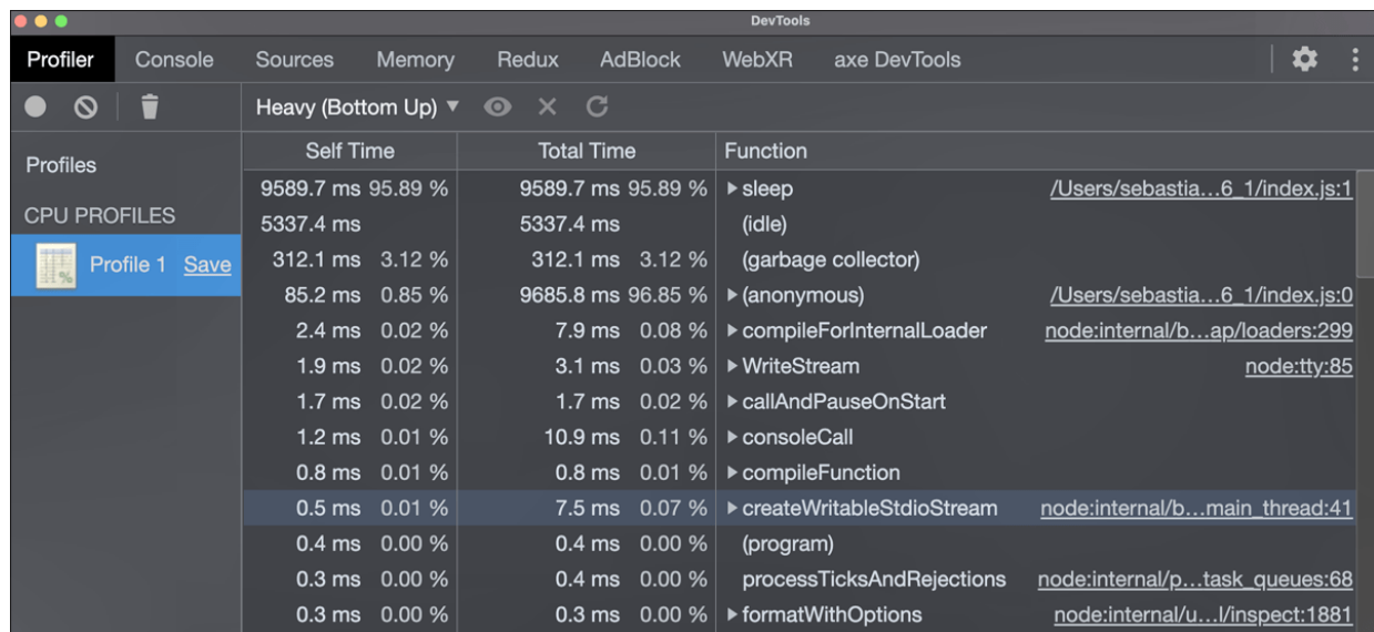
Figure 26.2 CPU Profiling with Chrome DevTools
