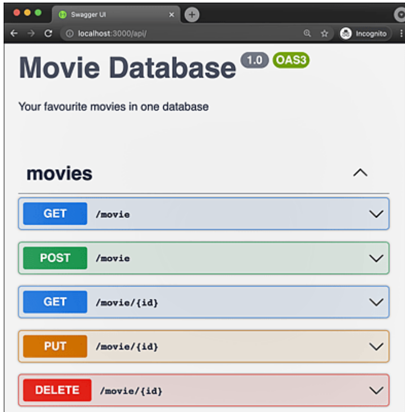
Figure 14.3 API Documentation of the MovieDB Application
