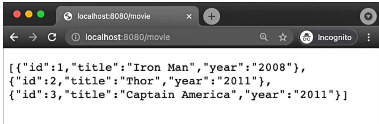
Figure 6.6 Movie List in the Browser
