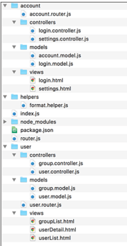
Figure 6.5 Structure for Extensive Applications
