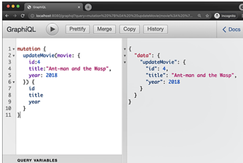
Figure 11.5 Modifying an Existing Data Record
