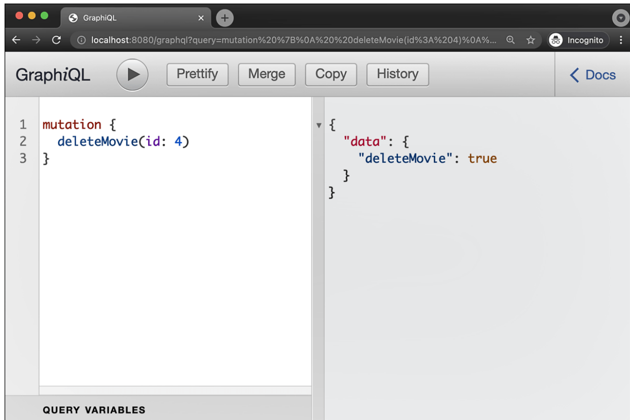
Figure 11.6 Deleting a Data Record
