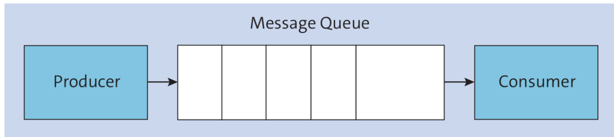
Figure 27.3 Message Queue
