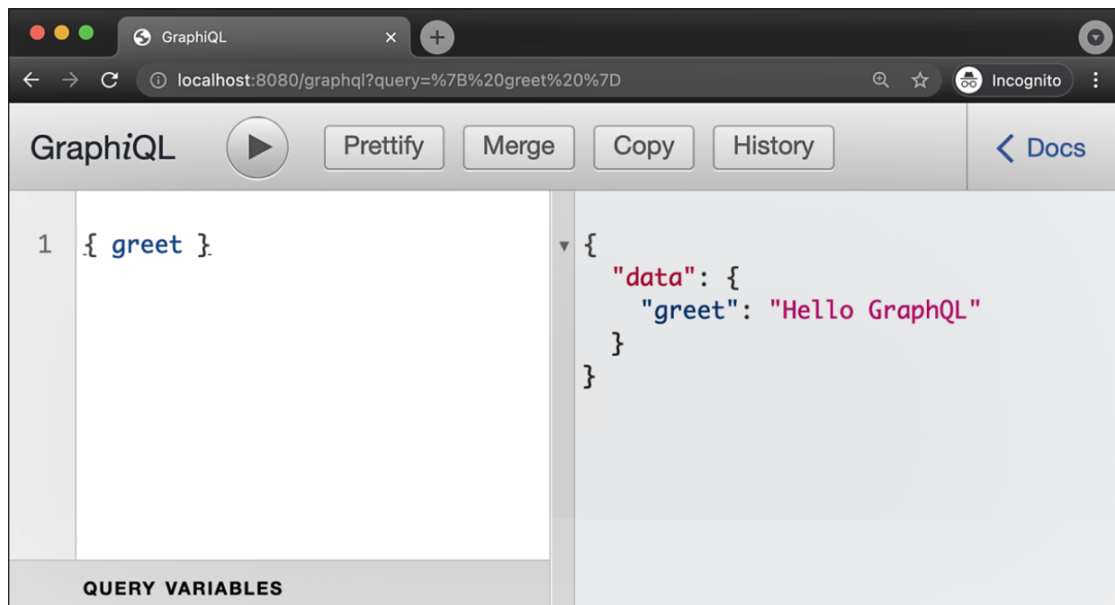
Figure 11.1 GraphiQL View
