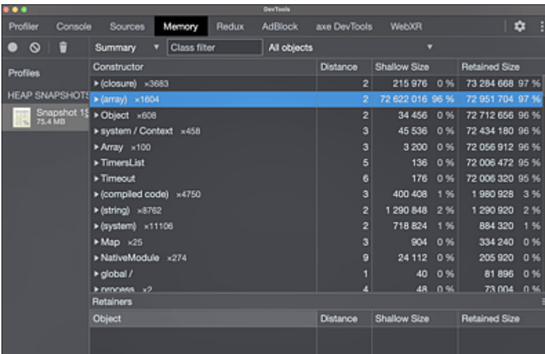
Figure 26.5 Heap Snapshot in DevTools
