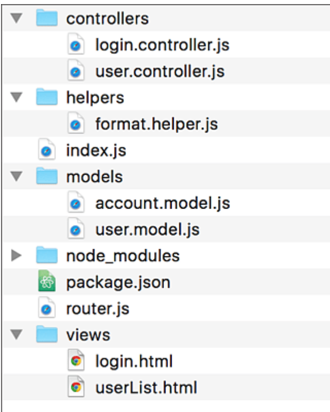
Figure 6.4 Structure for Medium-Size Applications
