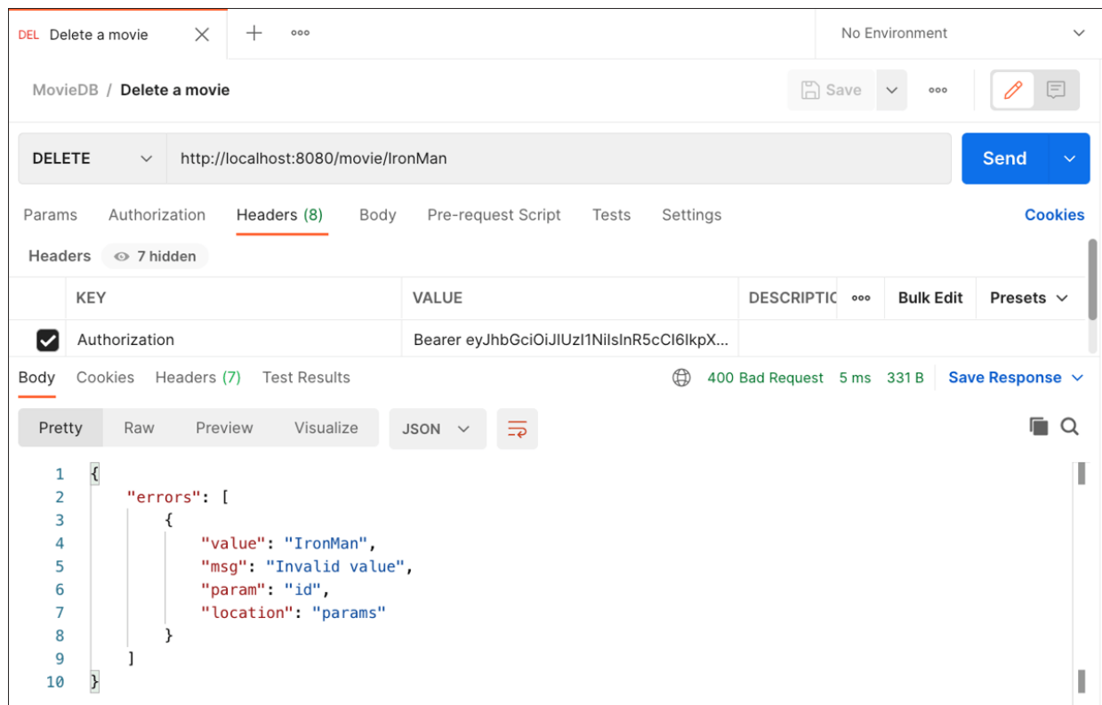
Figure 10.11 Invalid DELETE Request with Postman
