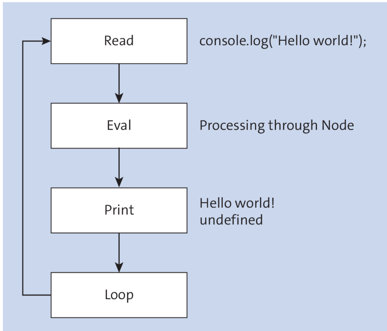
Figure 3.1 Interactive Mode of Node.js
