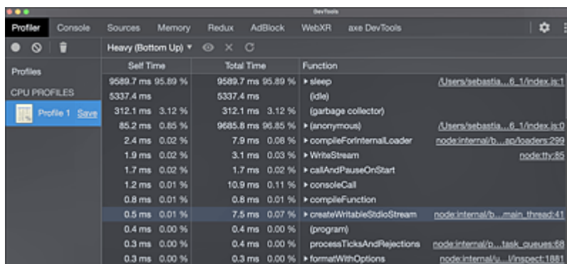
Figure 26.2 CPU Profiling with Chrome DevTools
