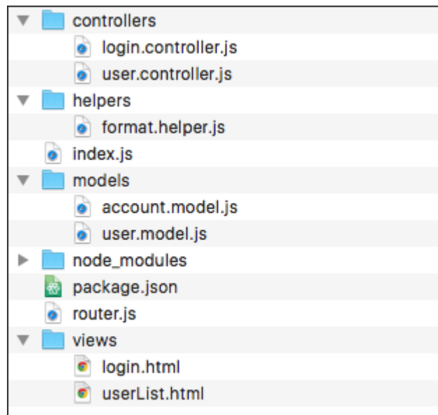
Figure 4.2 Structure of an Application
