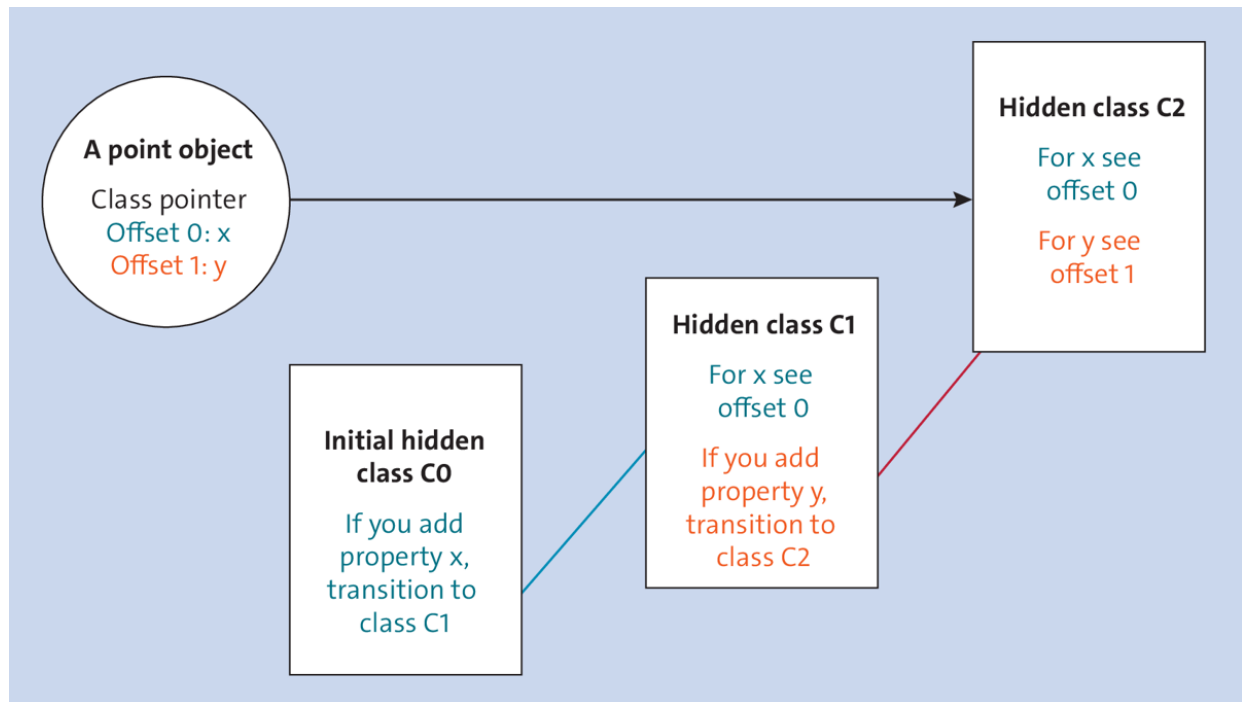
Figure 1.3 Hidden Classes in the V8 Engine ( https://github.com/v8/v8/wiki/Design%20Elements#fast-property-access )
