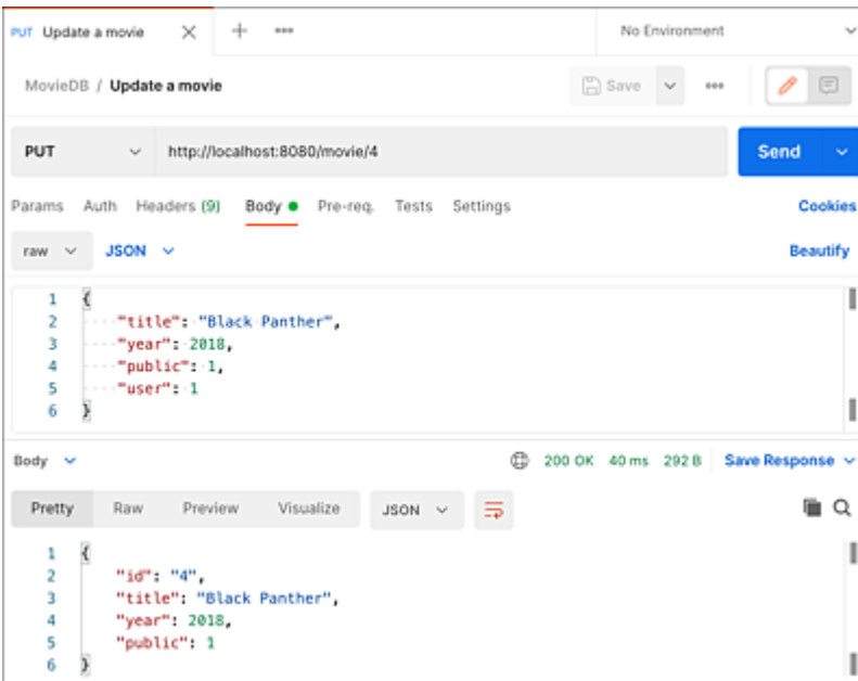
Figure 10.6 Updating a Data Record with Postman
