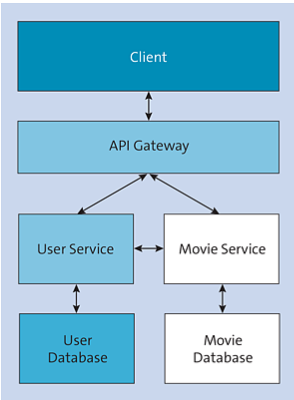
Figure 27.7 API Gateway in the Microservice Architecture
