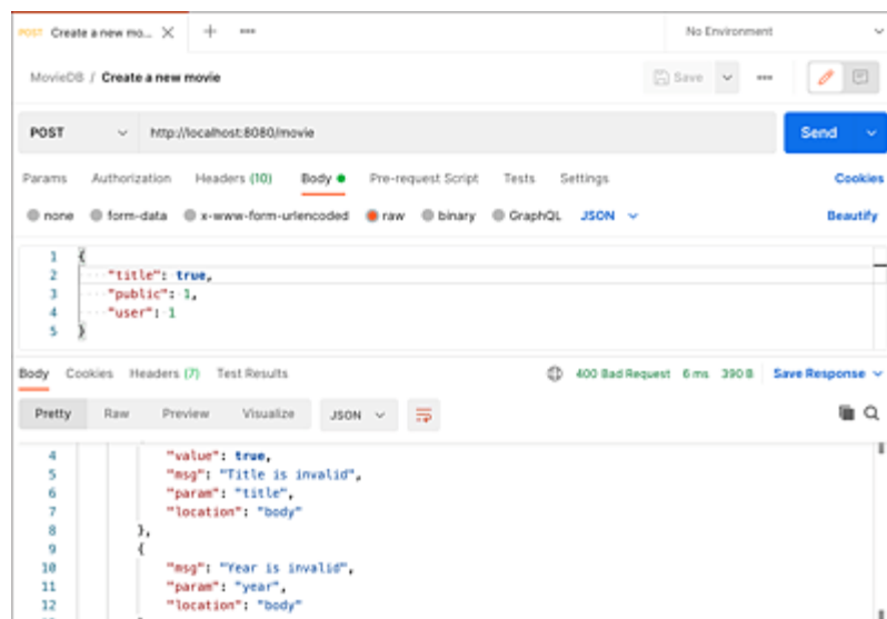
Figure 10.12 Incorrect Request with Postman
