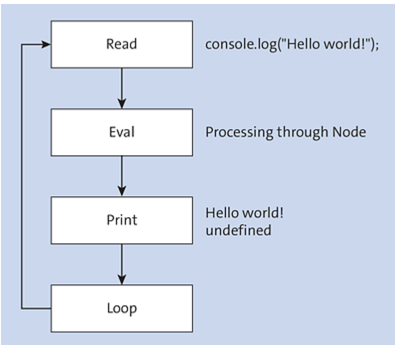
Figure 3.1 Interactive Mode of Node.js
