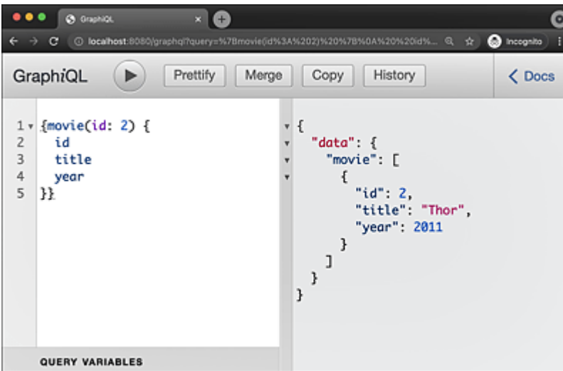
Figure 11.3 Querying a Data Record with GraphQL
