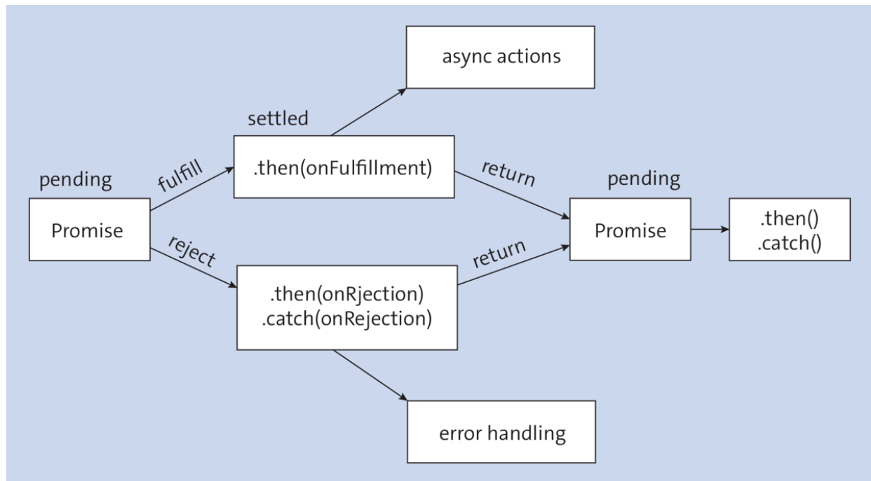
Figure 16.3 Lifecycle of a Promise
