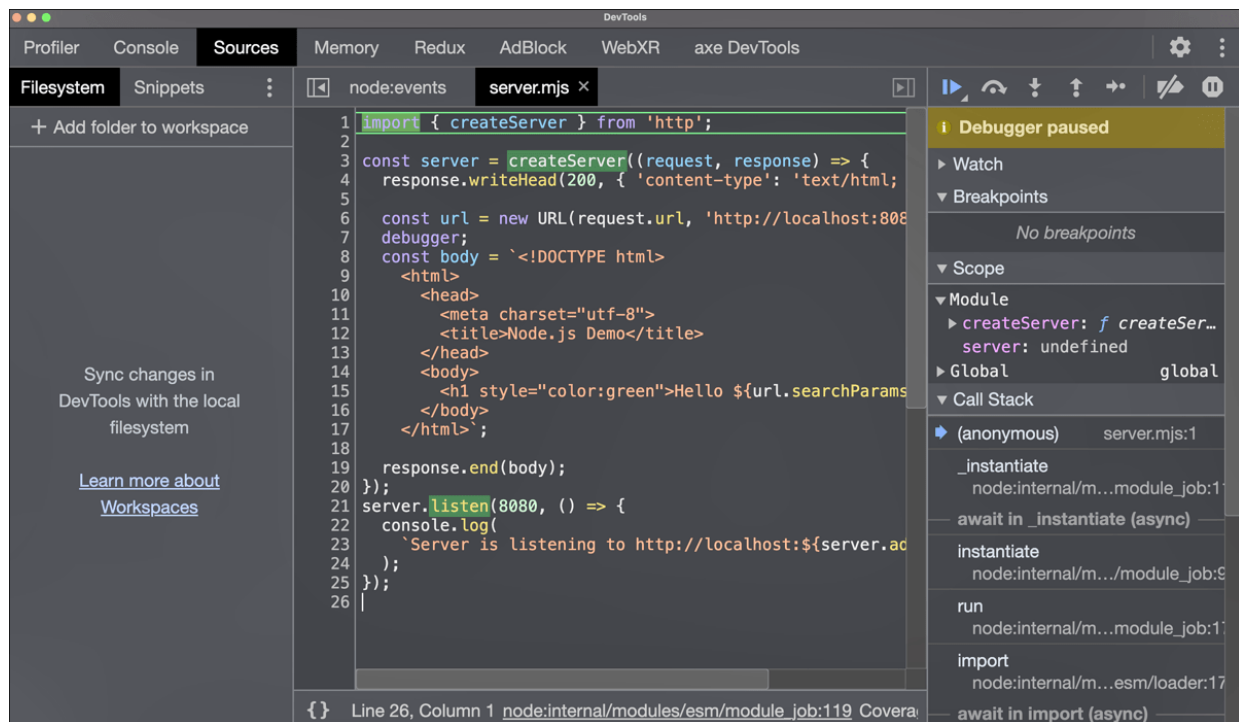
Figure 3.6 Active Debugging Session
