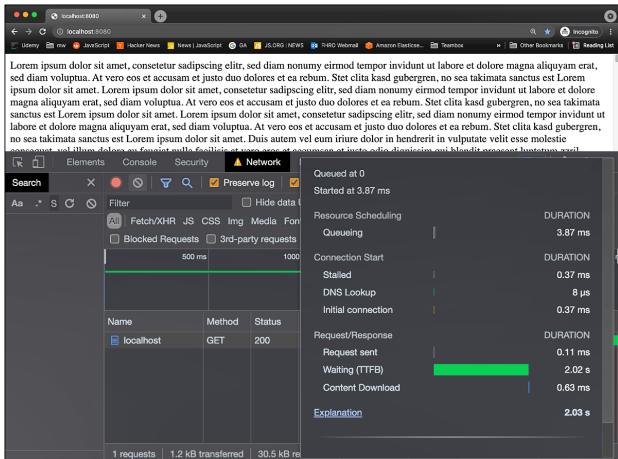
Figure 26.9 Measurement with Active Compression
