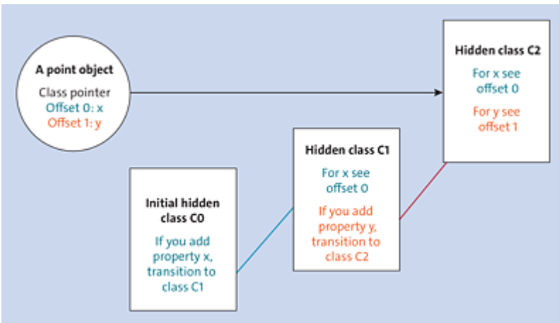
Figure 1.3 Hidden Classes in the V8 Engine ( https://github.com/v8/v8/wiki/Design%20Elements#fast-property-access )
