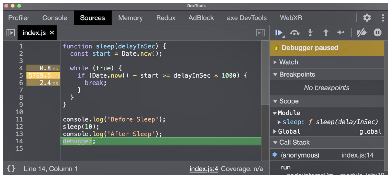
Figure 26.3 Display of Execution Time in DevTools
