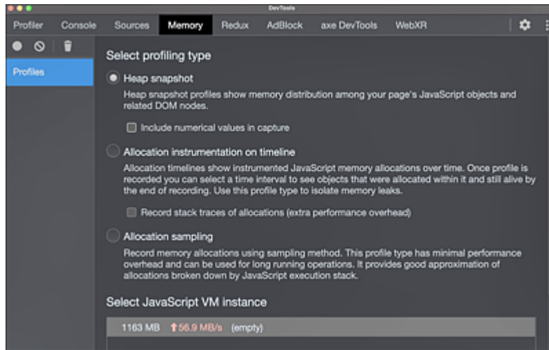
Figure 26.4 Current Memory Consumption and Trend Display
