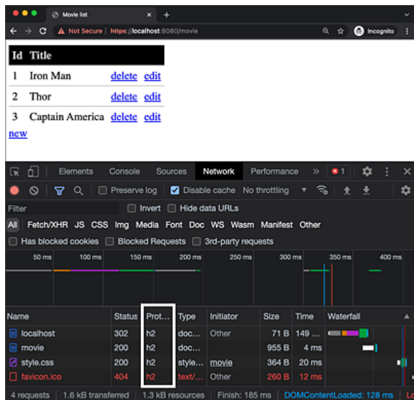
Figure 6.10 Delivery of Resources via the h2 Protocol
