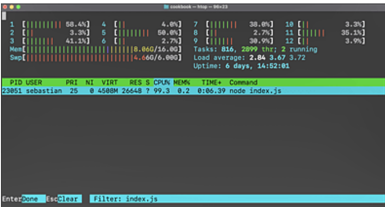
Figure 26.1 Output of “htop” for a CPU-Intensive Node.js Application
