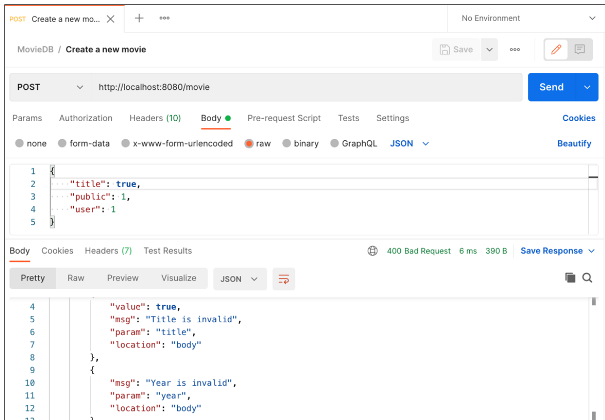
Figure 10.12 Incorrect Request with Postman
