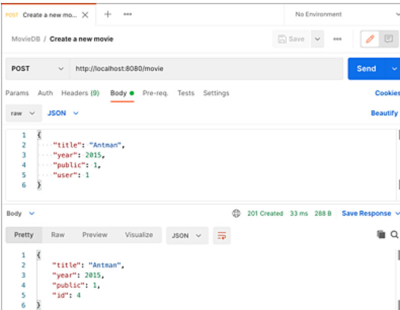
Figure 10.5 Creating a New Data Record with Postman
