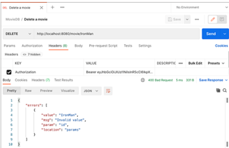
Figure 10.11 Invalid DELETE Request with Postman
