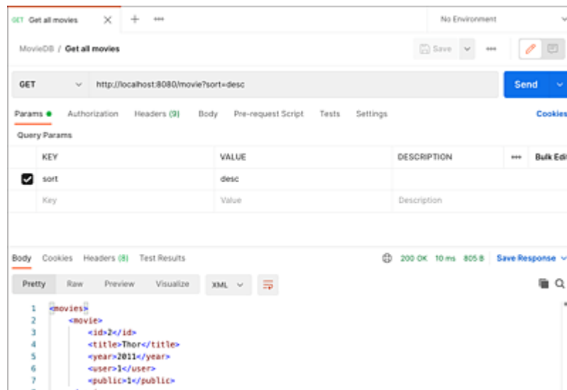
Figure 10.4 Sorting the Movie List with Postman
