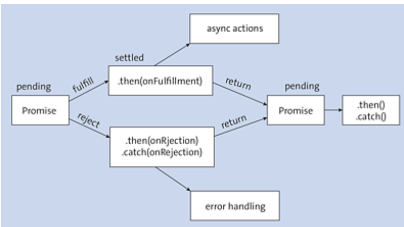
Figure 16.3 Lifecycle of a Promise
