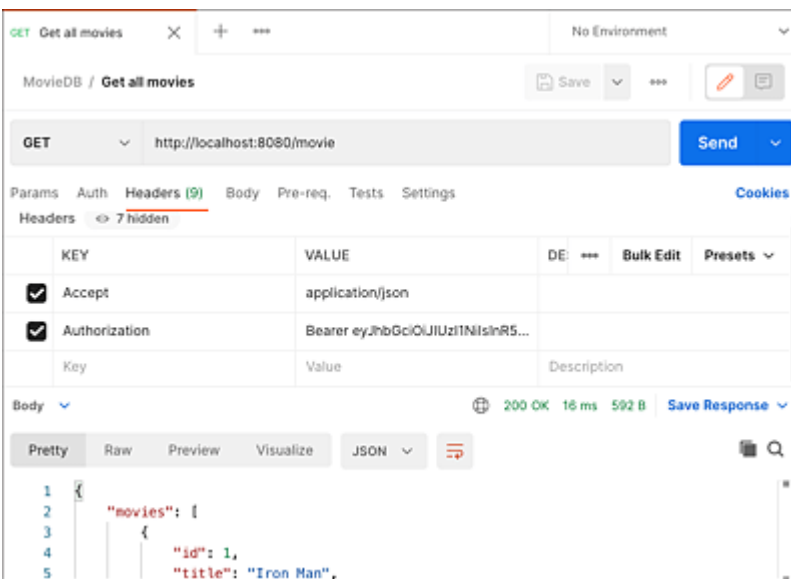
Figure 10.9 Read Request with Authorization Header in Postman
