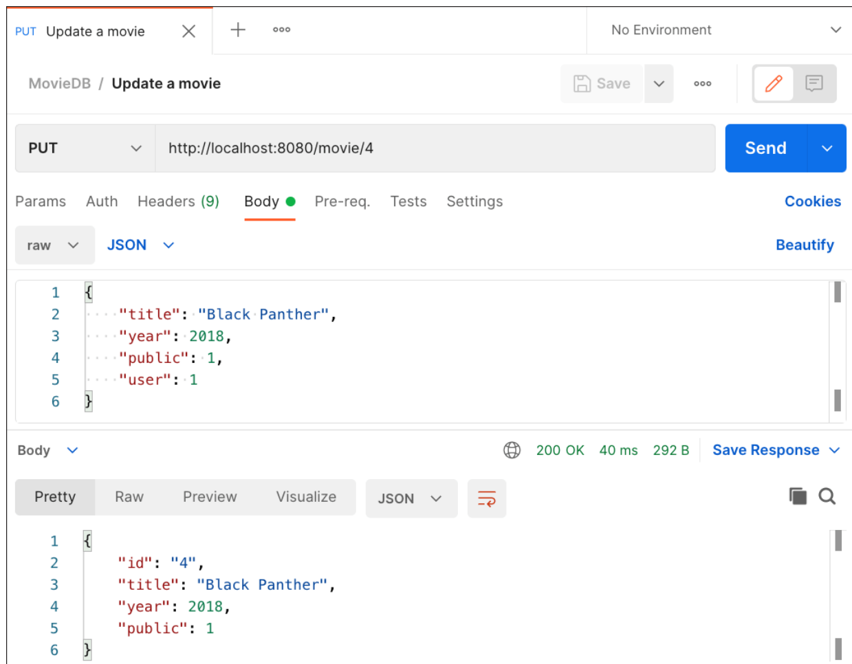
Figure 10.6 Updating a Data Record with Postman
