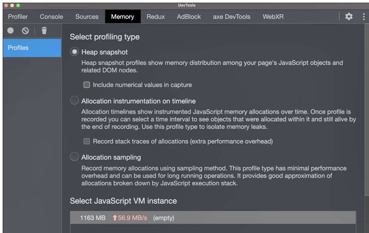
Figure 26.4 Current Memory Consumption and Trend Display
