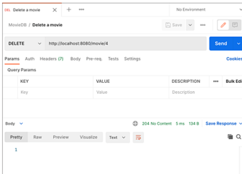
Figure 10.7 Deleting a Data Record with Postman
