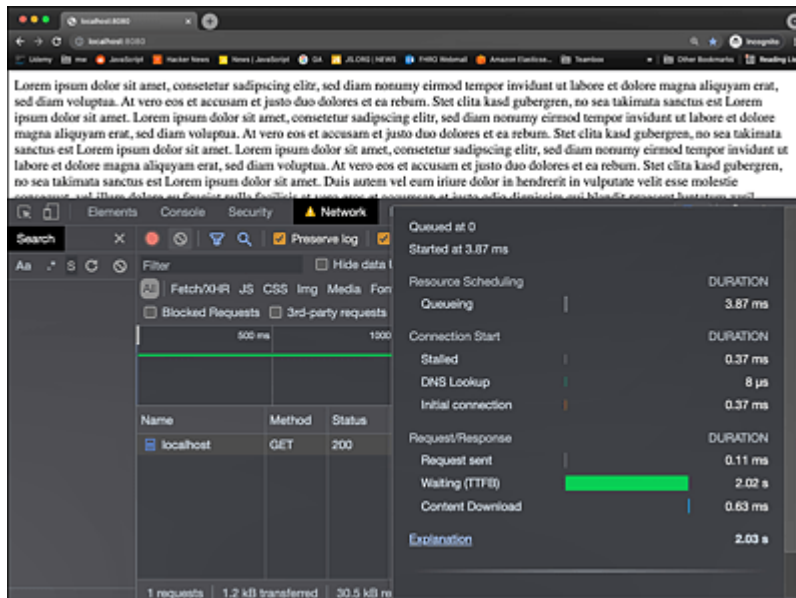
Figure 26.9 Measurement with Active Compression
