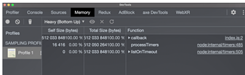
Figure 26.7 Memory Analysis with Allocation Sampling
