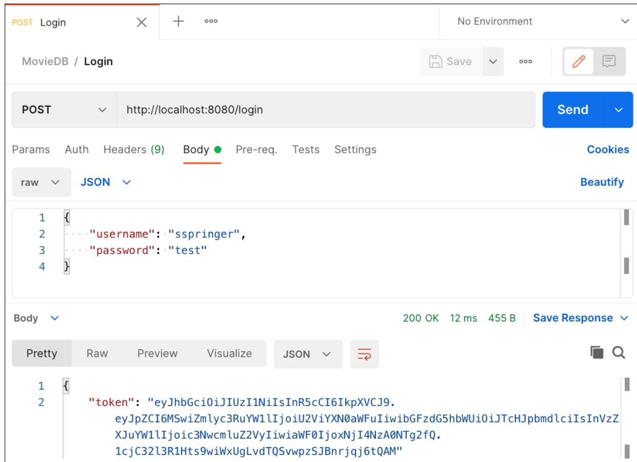
Figure 10.8 Login with Postman
