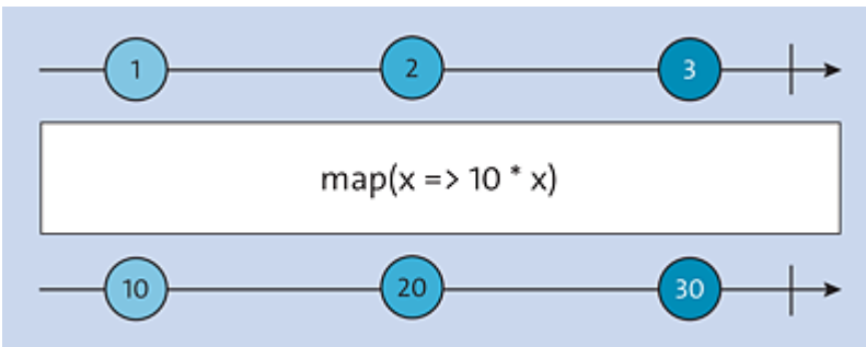
Figure 17.1 Marble Diagram for the “map” Operator
