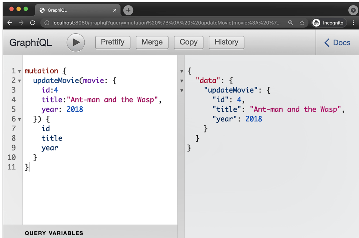
Figure 11.5 Modifying an Existing Data Record
