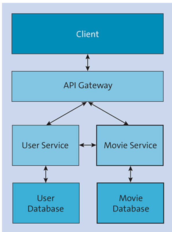
Figure 27.4 Architecture of the Sample Application
