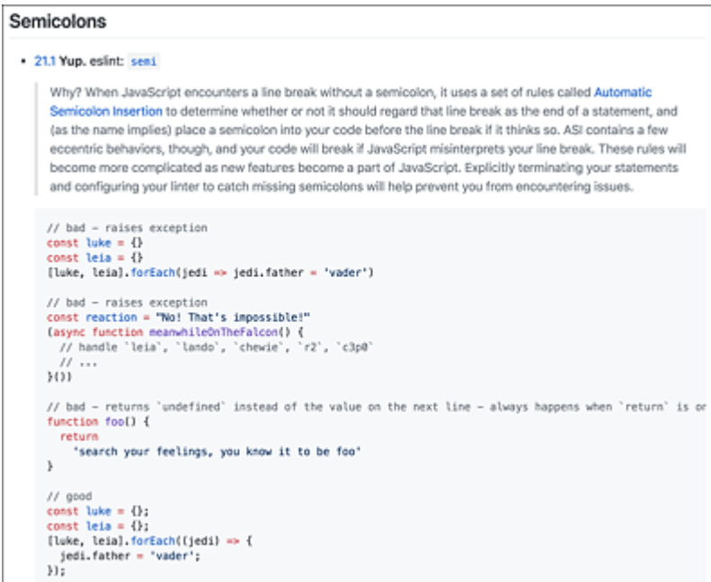
Figure 22.1 Airbnb Style Guide
