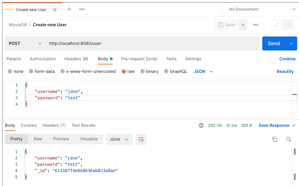
Figure 27.6 Creating a New User with Postman
