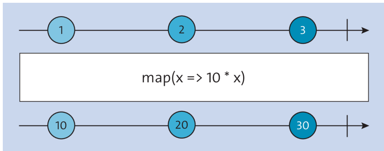
Figure 17.1 Marble Diagram for the “map” Operator
