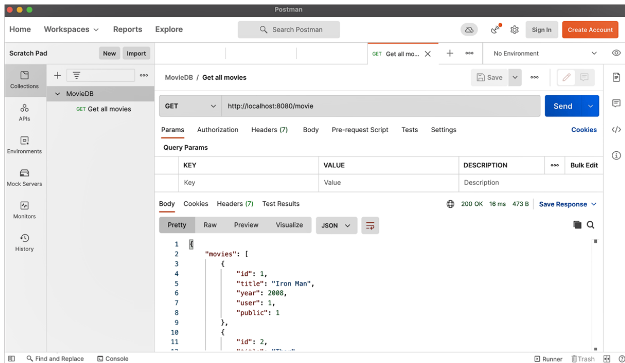
Figure 10.2 Querying Movie Records with Postman
