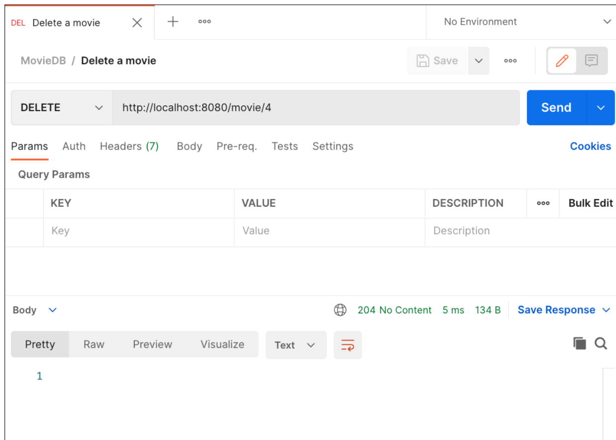
Figure 10.7 Deleting a Data Record with Postman
